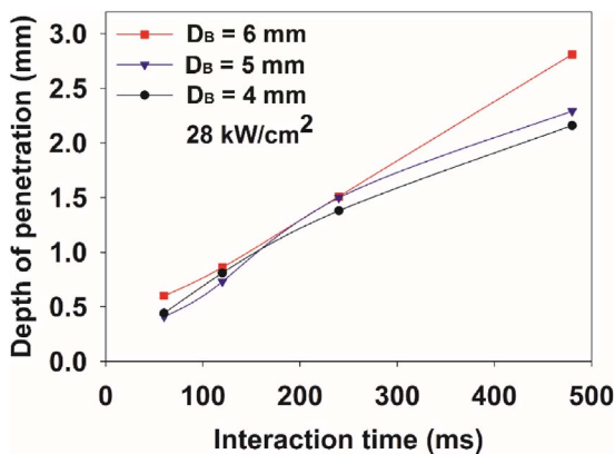
Fig. 7. Effect of interaction time on depth of penetration for different beam diameters and constant power density of 28 \text{ kW/cm}^2 (Table 2).
