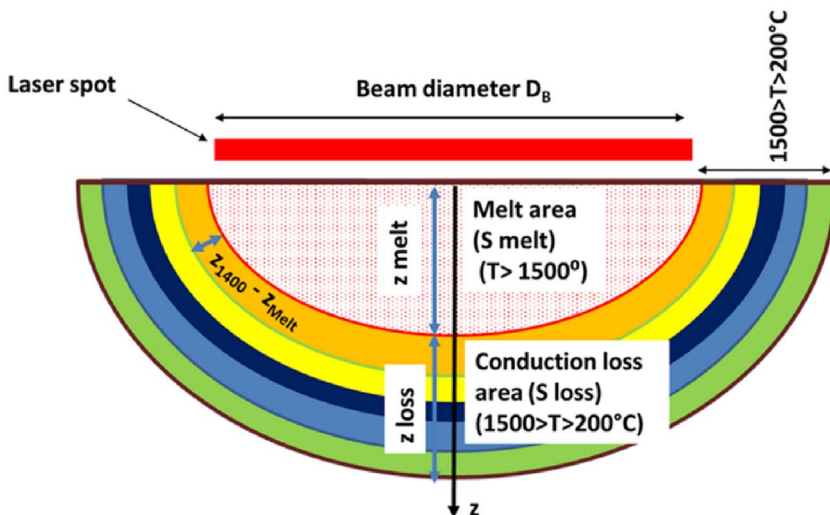
Fig. 2. Calculation of melt area and conduction loss area based on analytical solution of heat equation (Eq. (7)).
