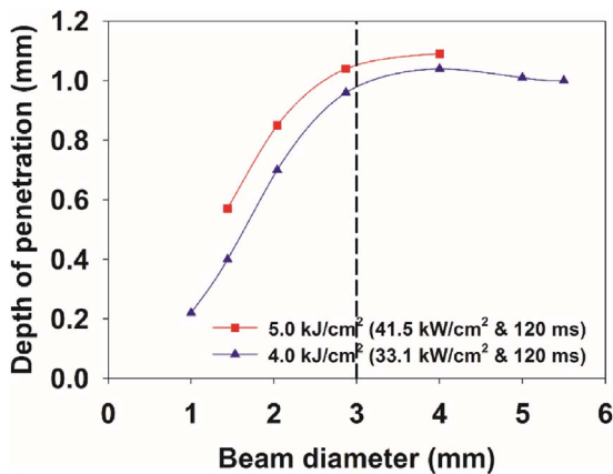
Fig. 11. Effect of beam diameter on depth of penetration at constant power density and interaction time.
