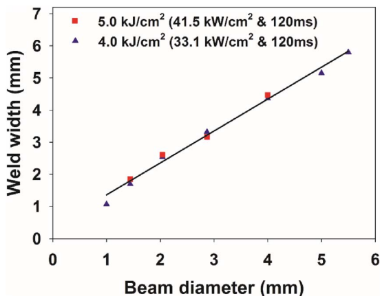
Fig. 12. Effect of beam diameter on weld width at constant power density and interaction time.
