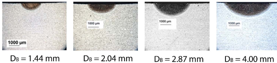
Fig. 10. Bead-on-plate welds produced at constant power density of 41.5 \text{ kW/cm}^2 and interaction time of 120 ms, for a range of beam diameters.
