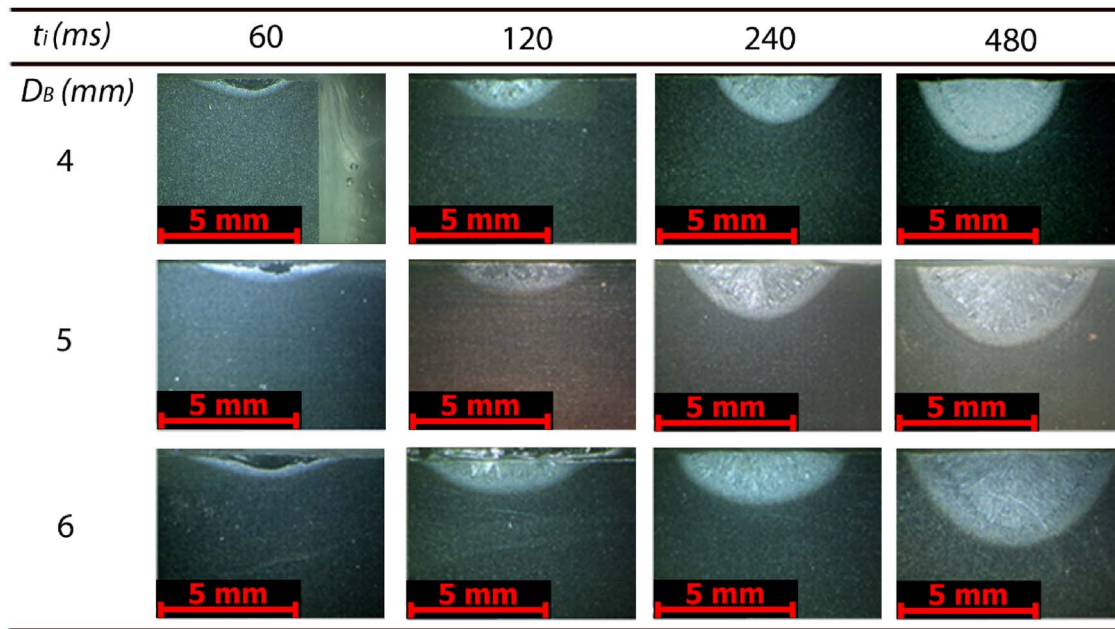
Fig. 6. Macrographs for different beam diameters and interaction times; constant power density of 28 \text{ kW/cm}^2 .
