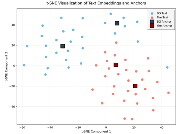
Fig. 3. CLIP based text embeddings for each class text and text-anchors after applying K-means clustering.
