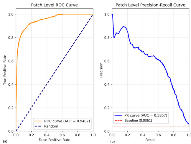
Fig. 4. ROC-AUC and PR-AUC curves for patch level classification in patch-head. (a) The patch-level ROC (AUC = 0.9487) shows strong discriminative ability. (b) The PR curve (AUC = 0.5857) remains well above the chance-level baseline (0.0361, corresponding to the ratio of positive to total samples). The relatively lower PR-AUC underscores the challenge of sustaining high precision in the presence of class imbalance.
