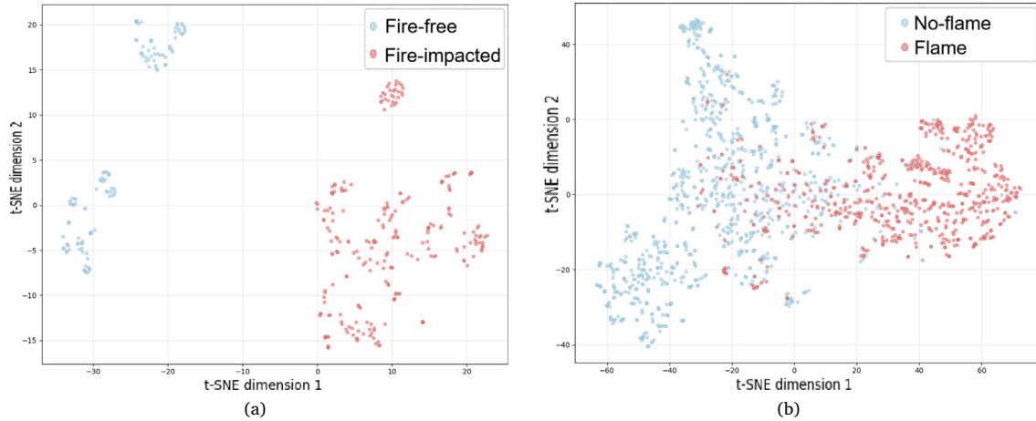
Fig. 5. t-SNE visualization of feature-embeddings (a) Image head (all test set images)(b) Patch head (randomly sampled 1500 patches from test set for better representation).
