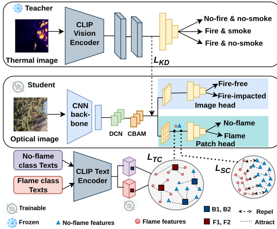
Fig. 2. Overall architecture for cross-modal knowledge distillation setup for wildfire detection and localization. Here, DCN is deformable convolutional network; CBAM is convolutional block attention module; B1 and B2 are two text-anchors for no-flame/background class; F1 and F2 are two text-anchors for the flame class. L_{KD} , L_{TC} , L_{SC} are knowledge distillation loss, text-based contrastive loss and supervised contrastive loss respectively given by Eqs. (13), (15) and (18).
