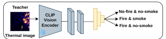
Fig. 1. Teacher model with frozen CLIP backbone and last two trainable layers. It is trained for a classification task using thermal images via cross entropy loss.
