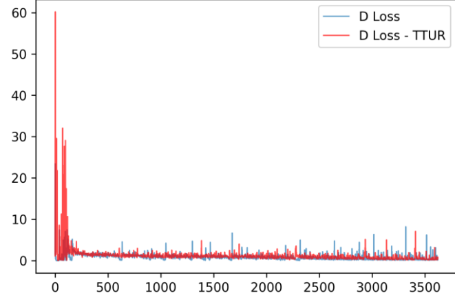
Fig. 4. Loss curves of two models trained using AdaS, the red one is that of the model implemented with TTUR while the blue one is that of the baseline model. TTUR increases the loss of D in the initial stages of training, indicating that G learns more.
