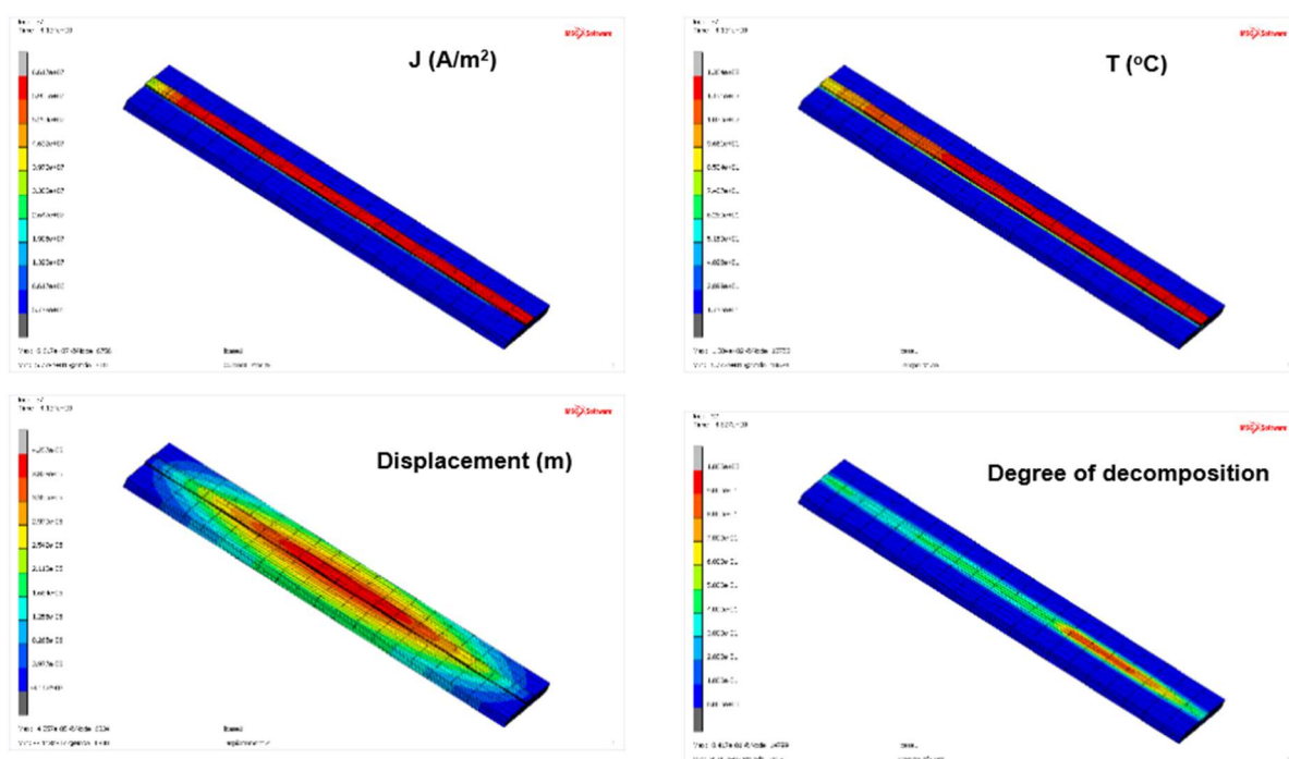
Figure 6 FE model of the electrothermal degradation simulation.
