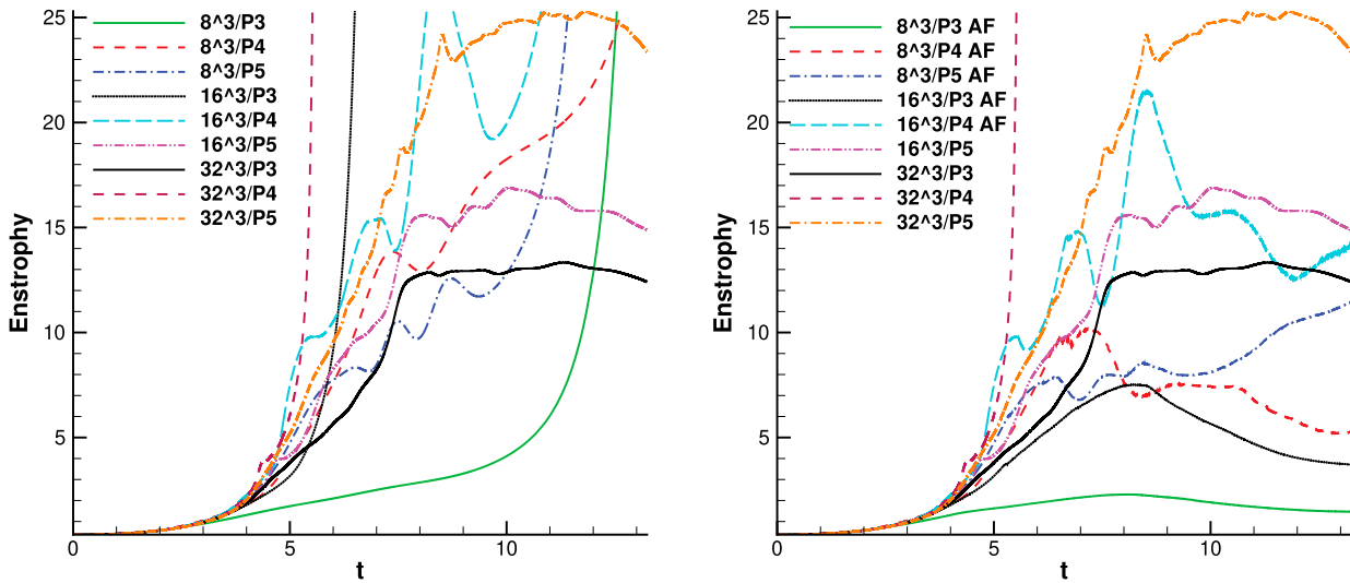
Figure 9. Enstrophy for unfiltered (left) and ADDA-DG (right). 16^3/P5 and 32^3 are unfiltered.
