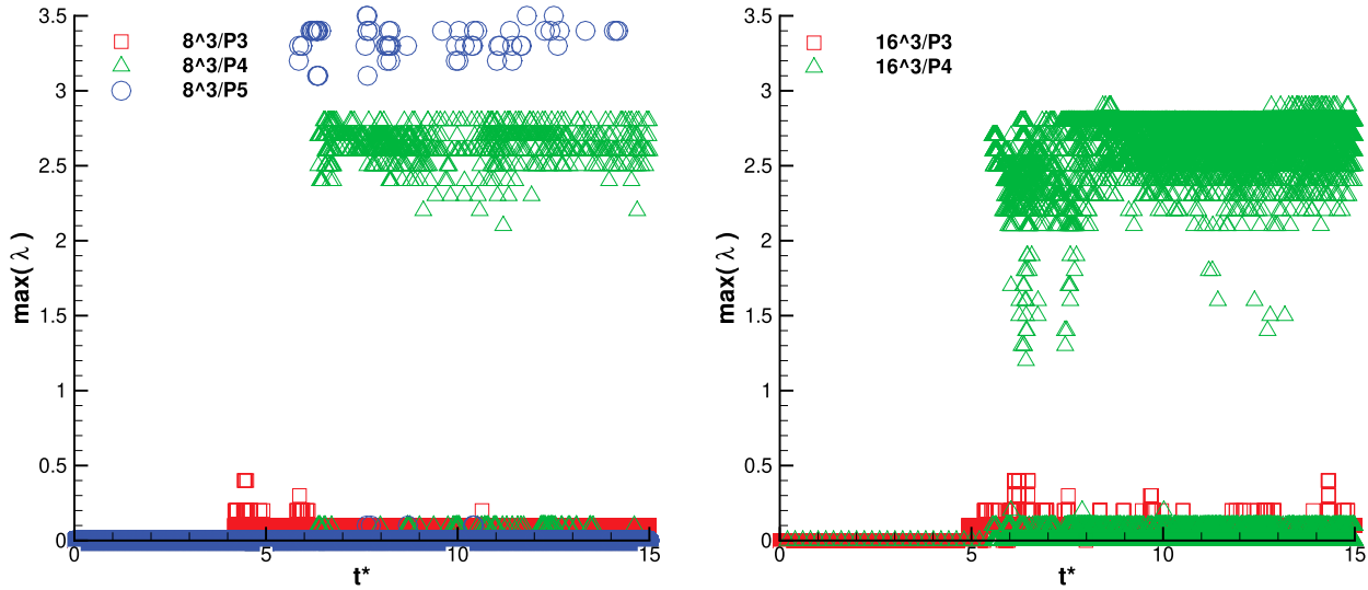
Figure 7. Maximum filter strength for AF-DG TGV on 8^3 and 16^3 hexahedral meshes. The \lambda value is the number of polynomial modes filtered, as detailed in Equation (22).
