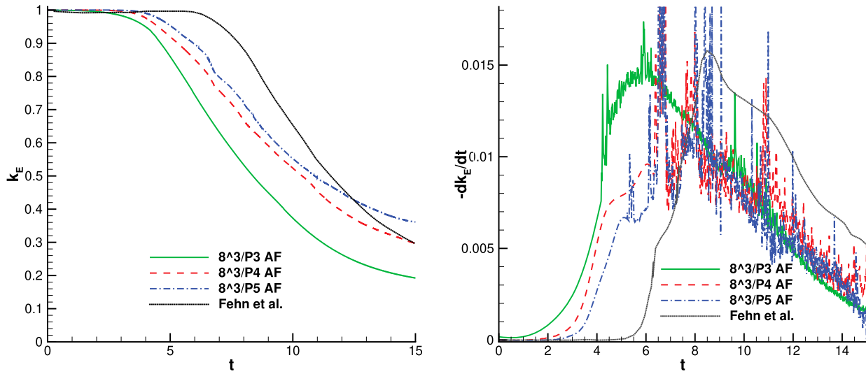
Figure 5. AF-DG TGV on an 8^3 hexahedral mesh, resolutions of \approx 22^3 , 26^3 , 31^3 , and 8192^3 , respectively.
