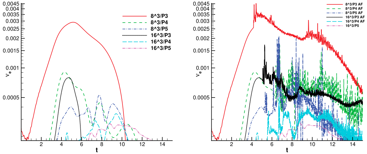
Figure 14. Effective viscosity \nu_e = -\frac{dk_\varepsilon}{dt}D^{-1} for unfiltered (left) and AF-DG (right). 16^3/P5 and 32^3 are unfiltered.
