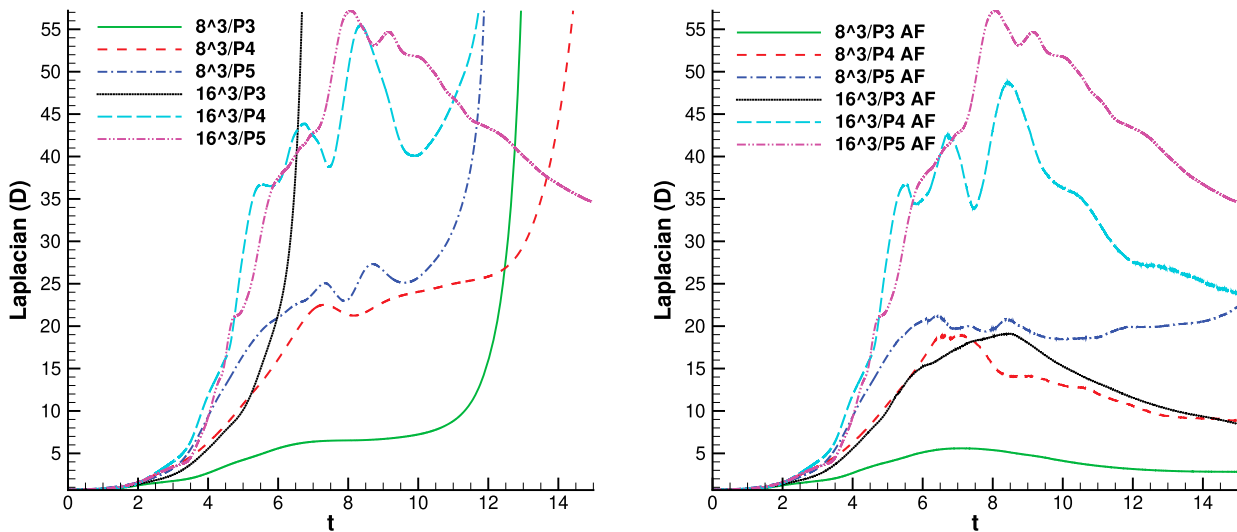
Figure 13. Laplacian term D for unfiltered (left) and AF-DG (right). 16^3/P5 and 32^3 are unfiltered.
