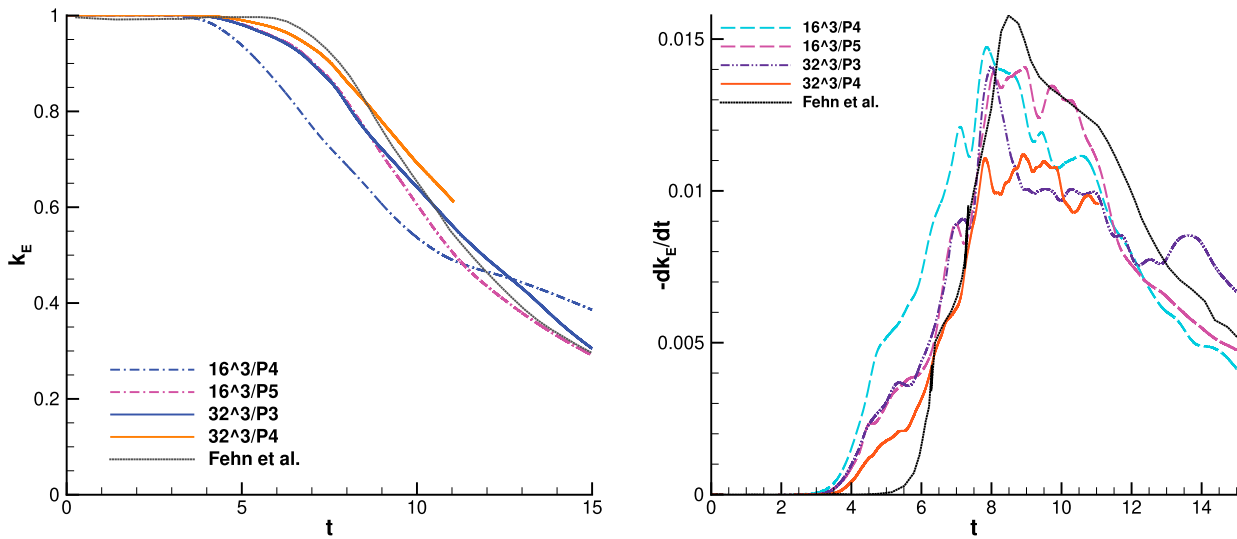
Figure 17. Unfiltered DG TGV with N + 1 quadrature order, resolutions of \approx 52^3, 61^3, 87^3, 105^3 , and 8192^3 , respectively.
