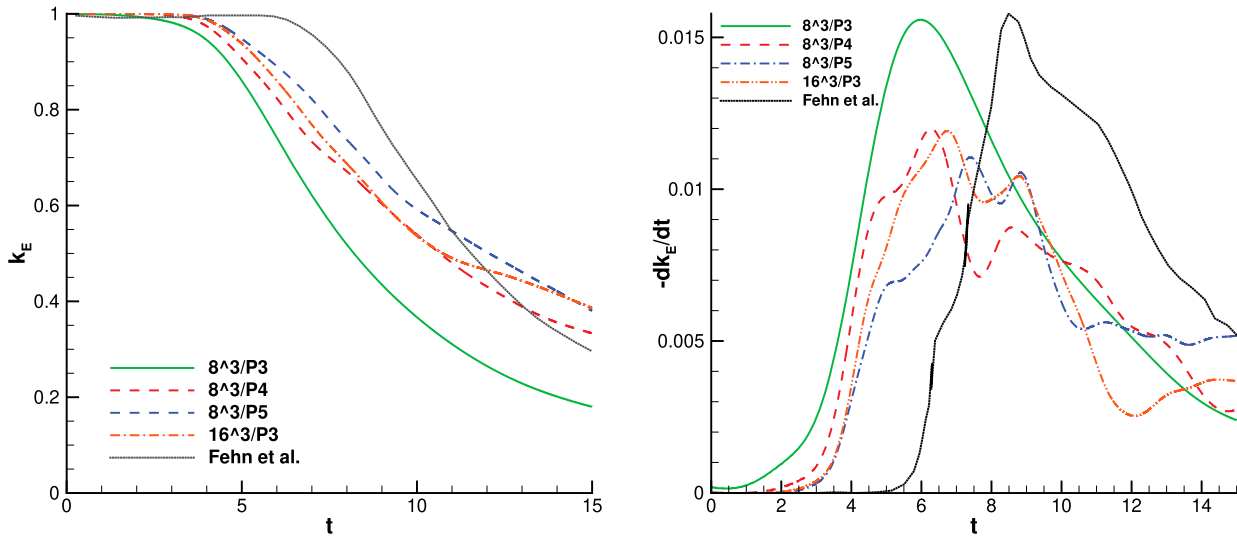
Figure 16. Unfiltered DG TGV with N + 1 quadrature order, resolutions of \approx 22^3, 26^3, 31^3, 43^3 , and 8192^3 , respectively.
