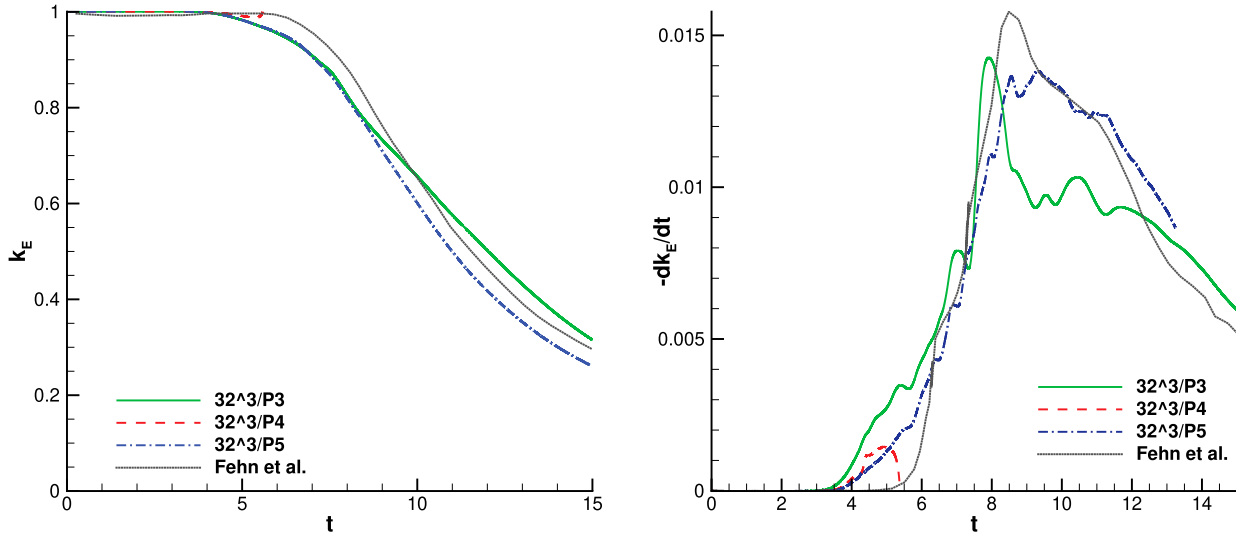
Figure 8. Unfiltered DG TGV on an 32^3 hexahedral mesh, resolutions of \approx 87^3, 105^3, 178^3, 864^3 , and 8192^3 , respectively.
