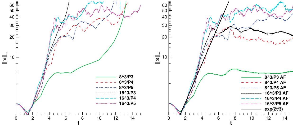
Figure 12. Maximum vorticity, semilog scale, for unfiltered (left) and AF-DG (right). 16^3/P5 and 32^3 are unfiltered.
