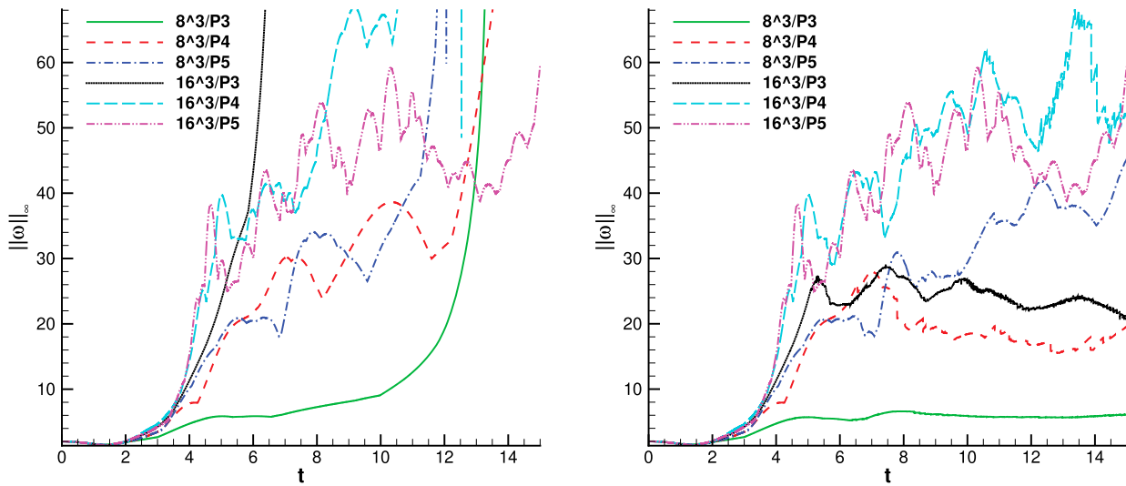
Figure 11. Maximum vorticity for unfiltered (left) and AF-DG (right). 16^3/P5 and 32^3 are unfiltered.
