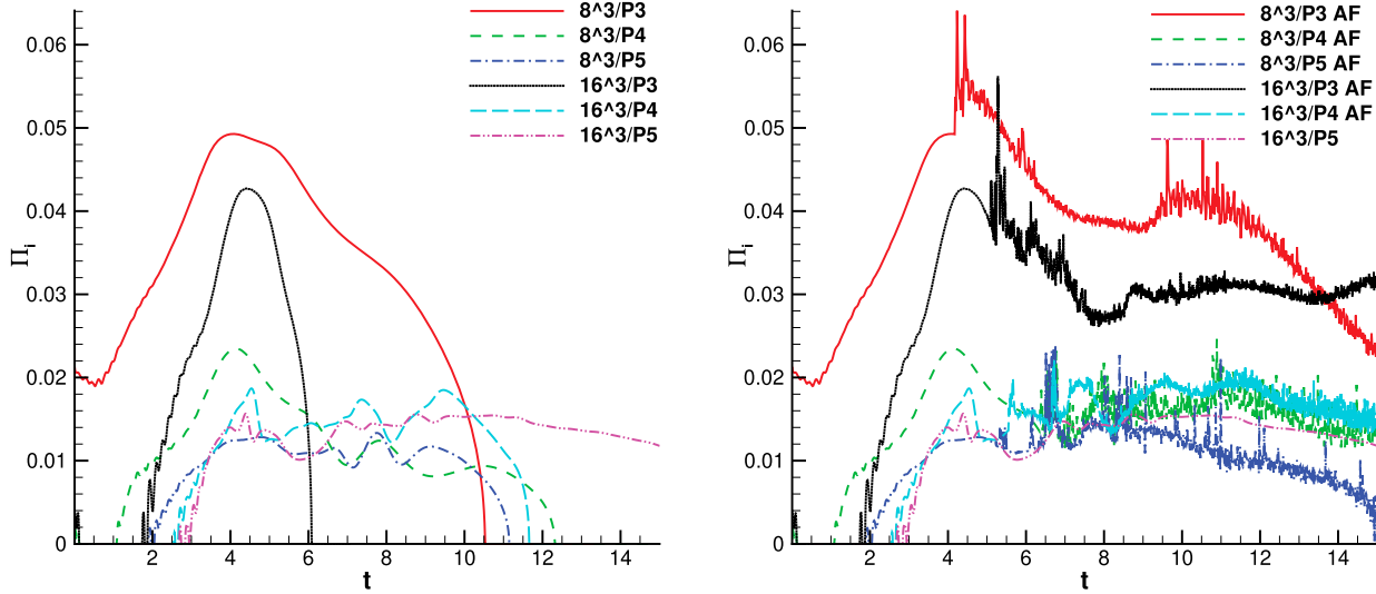
Figure 15. Dimensionless \Pi_l function for unfiltered (left) and AF-DG (right). 16^3/P5 and 32^3 are unfiltered.
