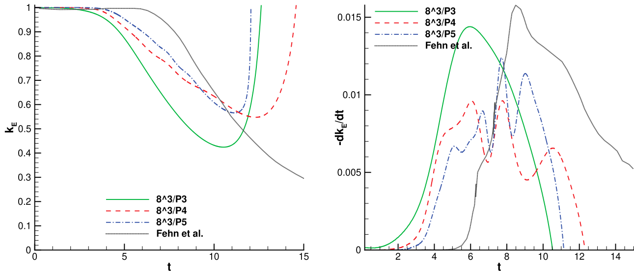
Figure 3. Unfiltered TGV on an 83 hexahedral mesh, resolutions of \approx 22^3 , 26^3 , 31^3 , and 8192^3 , respectively.
