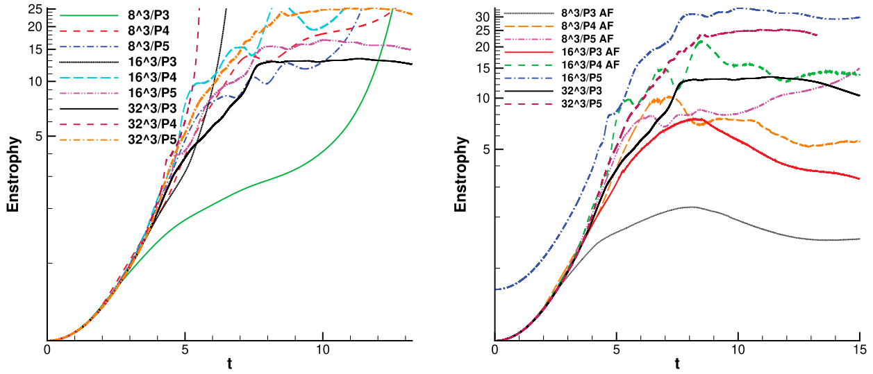
Figure 10. Enstrophy, semilog scale for unfiltered (left) and AF-DG (right). 16^3/P5 and 32^3 are unfiltered.
