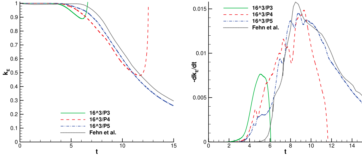
Figure 4. Unfiltered TGV on an 163 hexahedral mesh, resolutions of \approx 43^3, 52^3, 61^3 , and 8192^3 , respectively.
