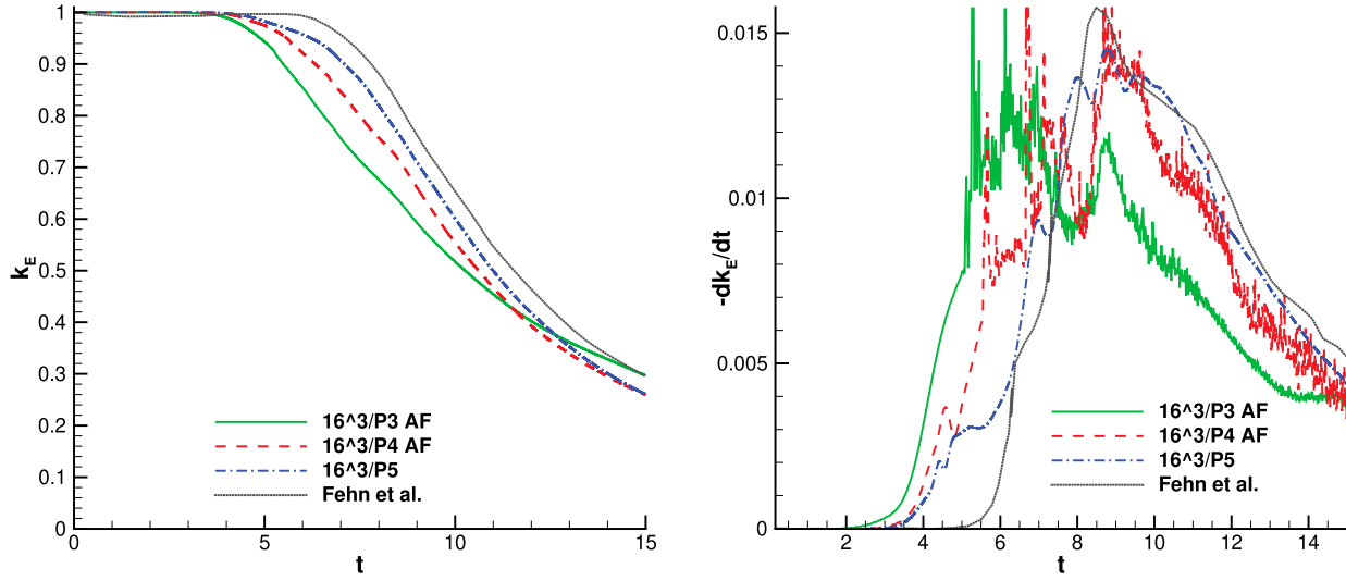
Figure 6. AF-DG TGV on an 16^3 hexahedral mesh, resolutions of \approx 43^3 , 52^3 , 61^3 , and 8192^3 , respectively.
