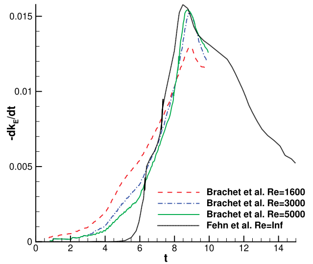
Figure 2. Reference DNS for TGV, resolutions of 2563, 2563, 8643, and 81923, respectively.
