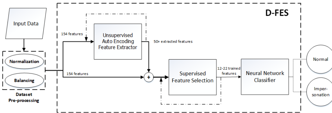
Fig. 1. Stepwise procedure of D-FES with two target classes: normal and impersonation attack
