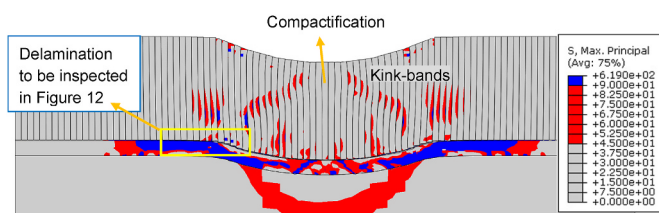
Fig. 9. Maximum principal stress computed with a 2D model of TBC after the impact of a spherical rigid particle with a diameter of 850 \mu\text{m} and speed of 100 m/s (units in MPa).
