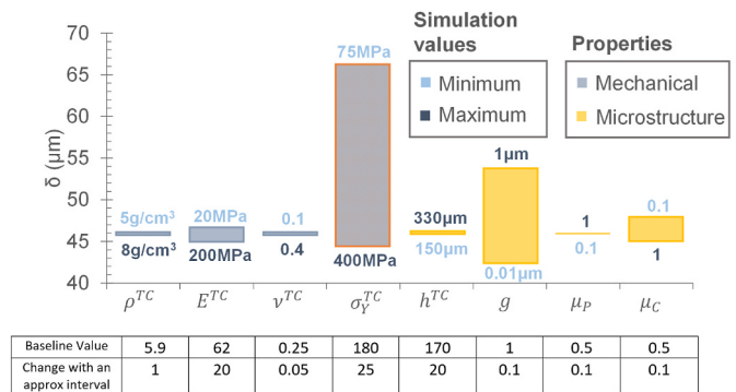
Fig. 7. Effects of each TC property on FOD penetration depth ( \delta ) quantified with the 2D model sensitivity tests with FOD particle of 850 \mu\text{m} diameter impacting at 100 m/s. Properties changed one at a time within an interval of change noted in blue. (For interpretation of the references to colour in this figure legend, the reader is referred to the Web version of this article.)
