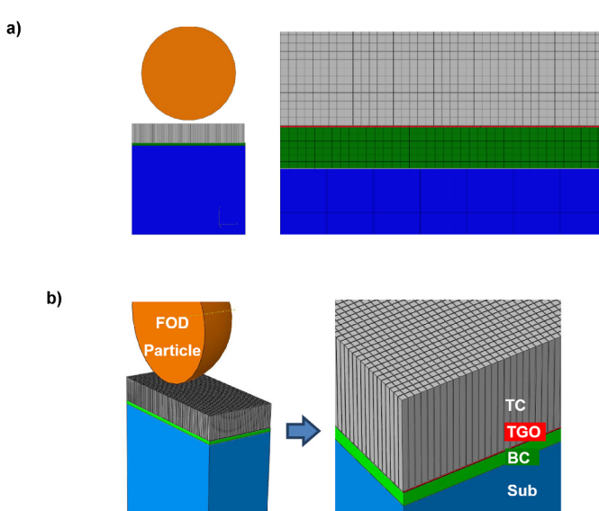
Fig. 5. FEM models represent a foreign object impacting a TBC with three layers. (a) 2D model, (b) 3D model. Note both the 2D and 3D models have employed the array of continuous columns to represent the EB-PVD TBC columnar microstructure.
