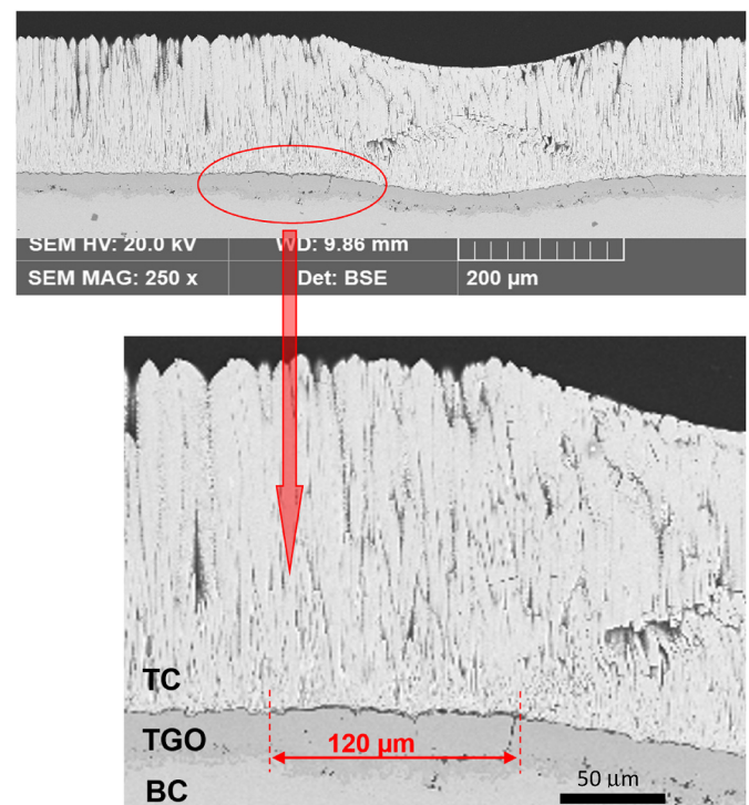
Fig. 11. Experiment measurement of the maximum length of delamination occurred at the TC/TGO or TGO/BC interfaces at one side of the TBC.
