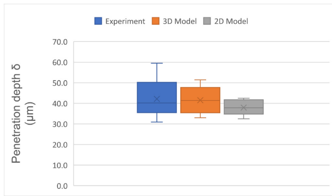
Fig. 8. Effects of Honite particle diameter (700–850 \mu\text{m} ) and speed (50–100 m/s) on FOD penetration depth ( \delta ) compared between experiment samples, 2D and 3D FEM models, showing a close match.
