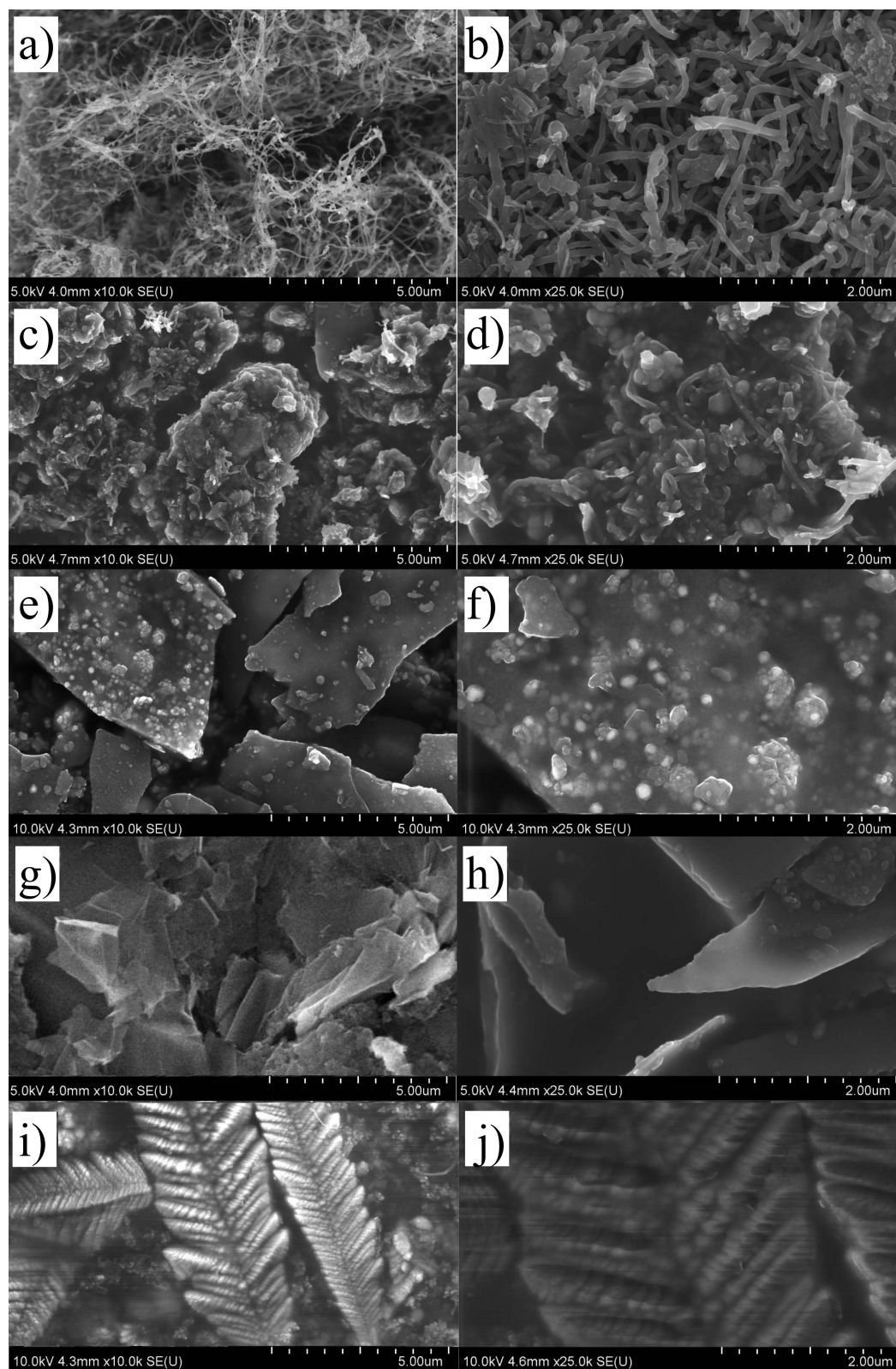
Figure 2 Scanning electron microscopy images of carbon structures synthesised with the usage of (a and b) cobaltocene, (c and d) magnesocene, (e and f) vanadocene, (g and h) ruthenocene, (i and j) manganocene as a catalyst. For each catalyst, images are presented at 10,000 \times (left) and 25,000 \times (right) magnification to allow consistent comparison of morphological features.
