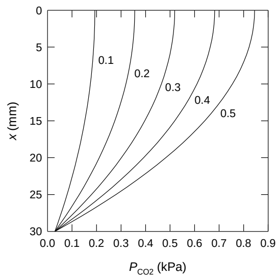
741 742 Fig. A1. Calculated \text{CO}_2 gradients through the experimental soil columns for different rates of 743 soil respiration (numbers on curves, units \text{mmol CO}_2 \text{ dm}^{-3} \text{ soil h}^{-1} ).
