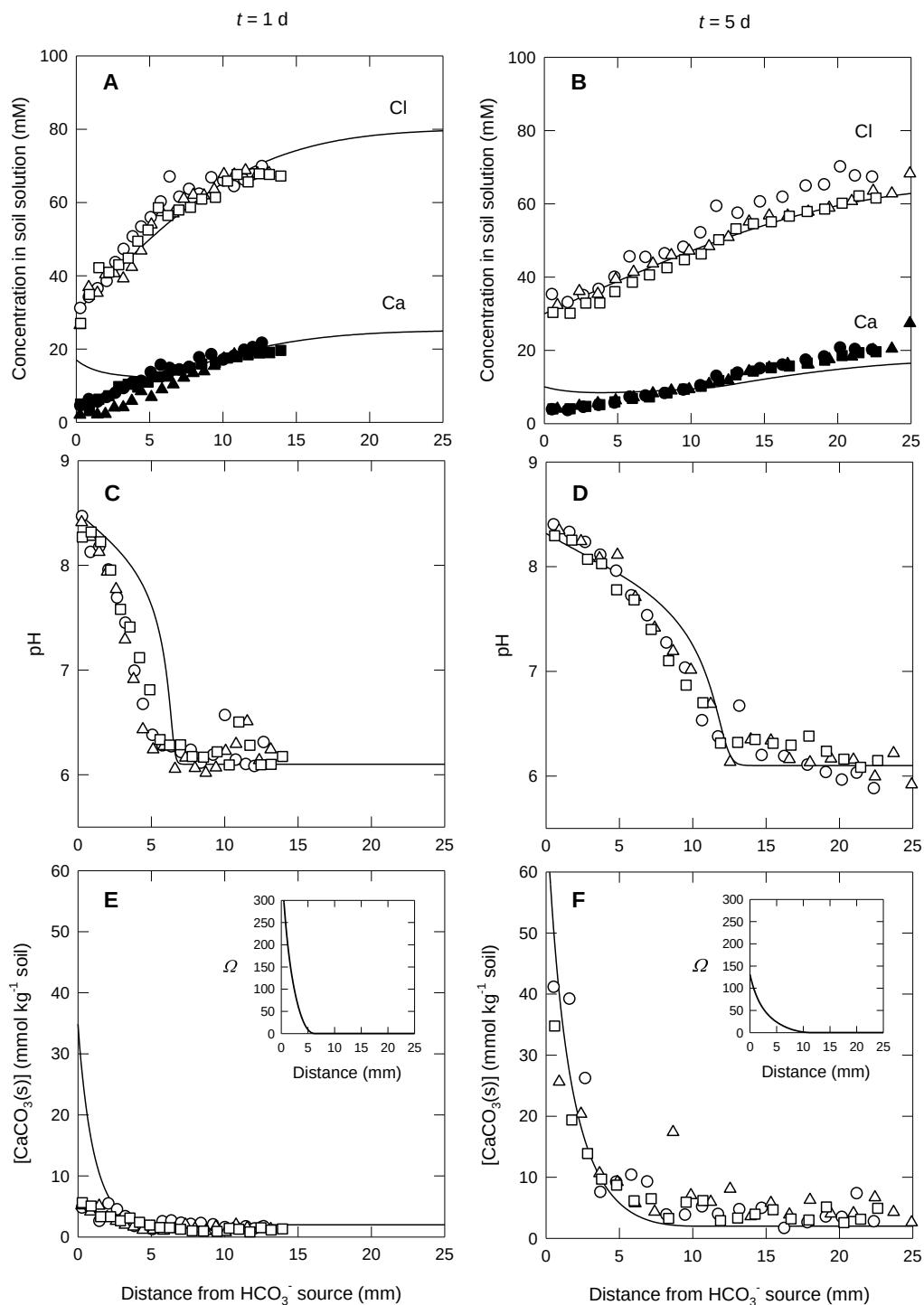
711 712 Fig. 2. Observed and calculated concentration profiles with distance from the resin-soil boundary. 713 The points are the measured values (three replicates indicated with different symbols). The lines 714 are the model predictions. The insets in the lower panels show the profiles of the calcite 715 saturation ratio ( \Omega = IAP/K_{sp} ).
