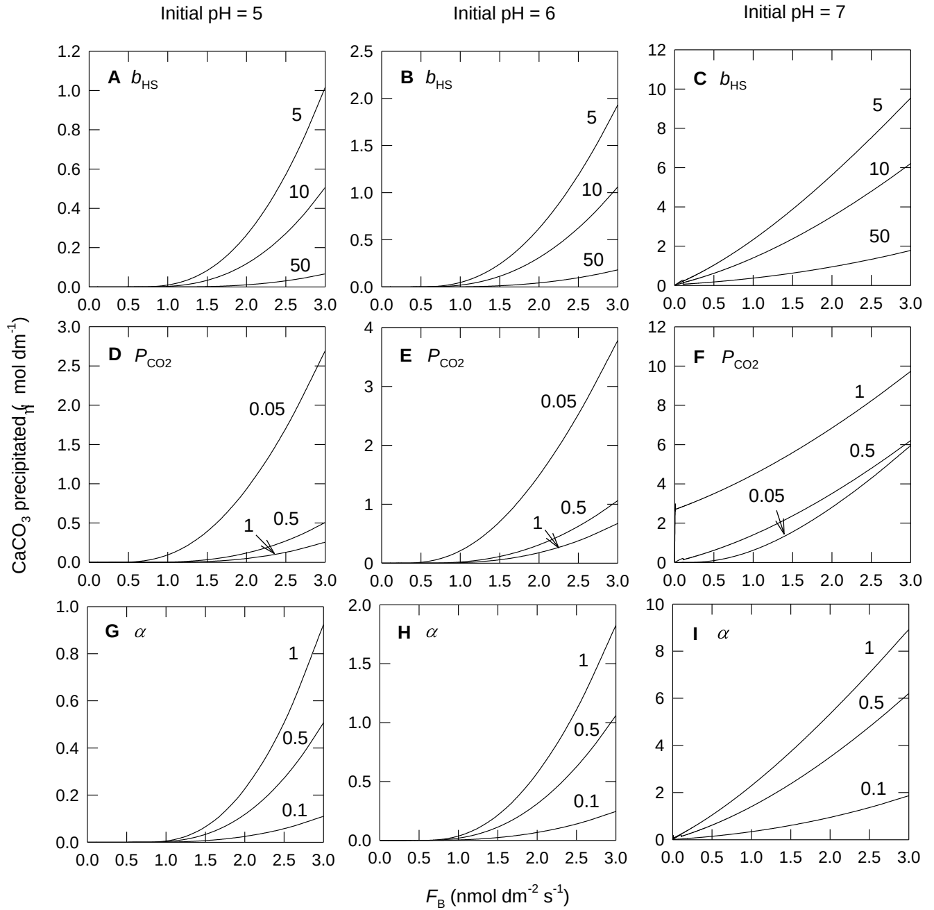
727 Fig. 4. Sensitivity analysis of the model in cylindrical geometry. The amount of CaCO 3 728 precipitated per unit length of cylinder of internal radius a is plotted against the flux of HCO 3 - 729 across a ( F_B ). The numbers on the curves are the values of the indicated variables. The effects of 730 (A-C) soil pH buffer power ( b_{\text{HS}} , \text{mmol dm}^{-3} \text{pH}^{-1} ), (D-F) CO 2 pressure ( P_{\text{CO}_2} , kPa) and (G-I) 731 precipitation rate constant ( \alpha , \text{nmol dm}^{-3} \text{s}^{-1} ). Other parameter values are: initial pH = 5, 6 and 7 732 (shown above panels); [\text{Ca}_{\text{total}}] set by Eq. (16); [\text{M}^+] = 30 \text{ mM} ; [\text{Cl}^-]_{\text{initial}} = 80 \text{ mM} ; a = 0.002 \text{ dm} ; 733 R = 0.052 \text{ dm} ; \rho = 1 \text{ kg dm}^{-3} ; \theta f = 0.02 ; t = 10 \text{ days} .
