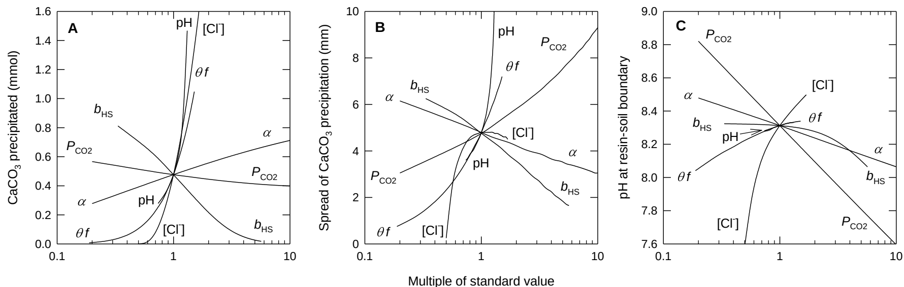
717 Fig. 3. Sensitivity analysis of the model in planar geometry. The output variables are: (A) the amount of CaCO 3 precipitated in the soil 718 column (obtained by numerical integration using Simpson's rule), (B) the spread of the CaCO 3 precipitation zone (obtained from the 719 distance at which [CaCO 3 (s)] falls to 5% of the value at the resin-soil boundary) and (C) the pH at the resin-soil boundary. Each of the 720 indicated input variables is varied in turn with the other variables at their standard values (e.g., \alpha varies from 0.2 to 10 \times its standard value). 721 Note x-axis is logarithmic. The ranges in input values (standard values in parenthesis) are: \theta (soil water content) = 0.1–0.8 (0.53), f (diffusion 722 impedance factor) = 0.5 \theta (Kirk 2004), pH initial = 4.5–8 (6.1), [Cl - ] initial = 40–135 (80) mM, P_{CO_2} = 0.1–5 (0.5) kPa (Kirk, 2004), b_{HS}^* (pH 723 buffer power) = 4–85 (15) mmol kg -1 pH -1 (Corstanje et al. 2008), \alpha^* (precipitation rate constant) = 0.1–5 (0.5) nmol kg -1 s -1 (Section 4.2.3). 724 Time = 5 d. *Per unit soil mass basis
