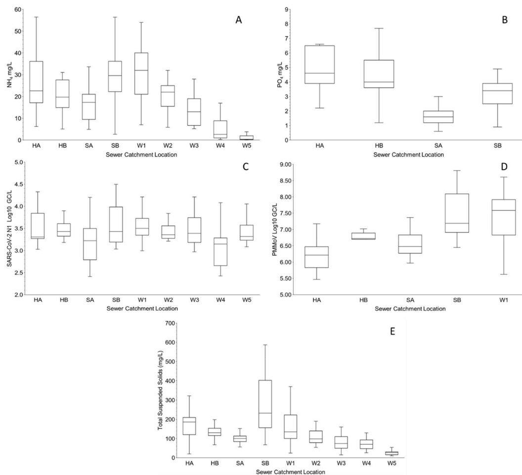
Fig. 4. A) \text{NH}_4\text{-N} mg \text{L}^{-1} , B) \text{PO}_4\text{-P} mg \text{L}^{-1} , C) SARS-CoV-2 N1 Log10 GC/L, D) PMMoV Log10 GC/L and E) TSS mg \text{L}^{-1} at sewershed sample points. N.B: HA – Halls of Residence A, HB – Halls of Residence B, SA – Technical In-Sewer, SB – Residential In-Sewer, W1 – Influent, W2 – Post Primary Lamella, W3 – Post Roughing Trickling Filter, W4 – Post Secondary Trickling Filter and W5 – Final Effluent.
