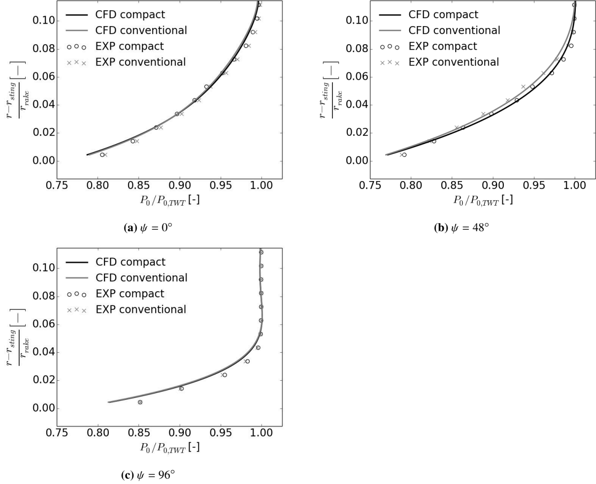
Fig. 9 Boundary layer profiles at the rake location for selected azimuthal locations at mid-cruise conditions ( M = 0.85 , MFCR = 0.7 and \alpha_{nac} = 4.5^\circ )
