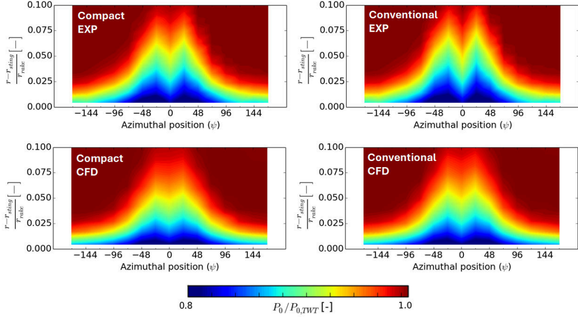
Fig. 8 Azimuthal changes of total pressure ratio at the rake location for mid-cruise conditions ( M = 0.85 , MFCR = 0.7 and \alpha_{nac} = 4.5^\circ )
