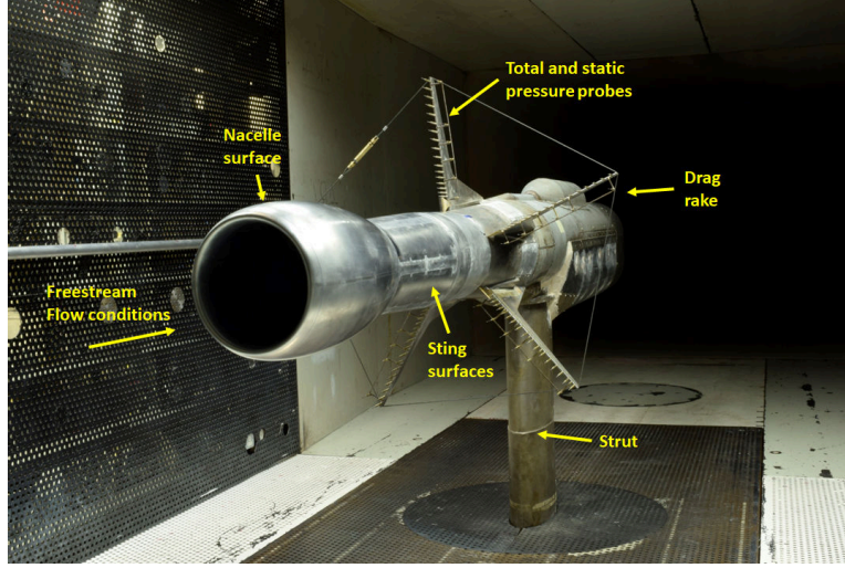
Fig. 1 Front view of the ARA Z30 large scale nacelle test rig
