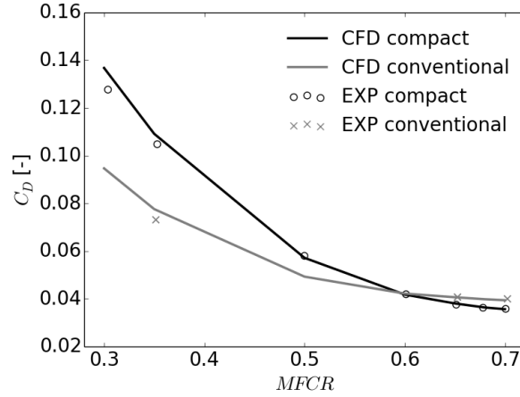
Fig. 12 Nacelle drag coefficient as a function of MFCR at fixed M = 0.84 and \alpha_{nac} = 4.5^\circ
