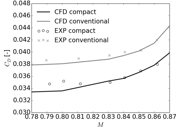
Fig. 10 Nacelle drag coefficient as a function of Mach number at fixed MFCR = 0.7 and \alpha_{nac} = 4.5^\circ
