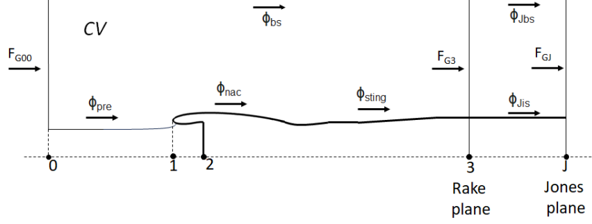
Fig. 3 Schematic of the thrust-drag bookkeeping method
