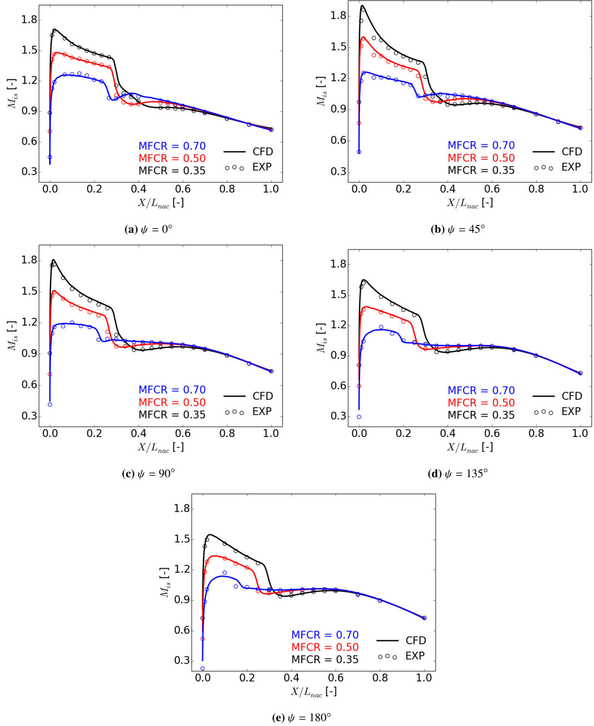
Fig. 13 Isentropic Mach number distribution along the compact nacelle ( L_{nac}/r_{hi} = 3.1 ) as a function of MFCR at fixed M = 0.84 and \alpha_{nac} = 4.5^\circ
