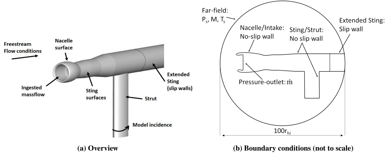
Fig. 2 Computational model of the ARA Z30 nacelle test rig
