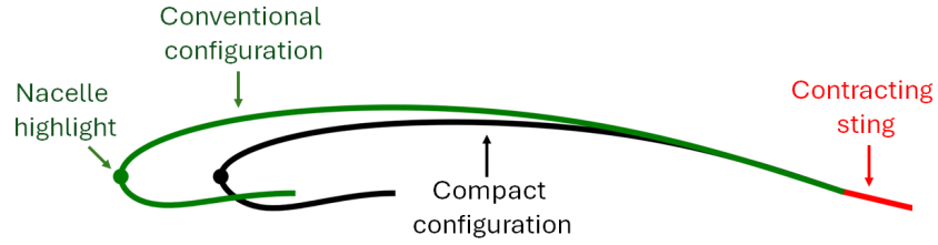
Fig. 5 Comparison of the side aero-line ( \psi = 90^\circ ) of both downselected nacelles. The initial shape of the sting for the wind-tunnel arrangement is also presented for reference
