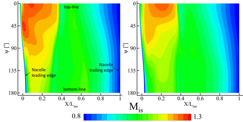
Fig. 4 Computed unwrapped surfaces of the nacelle: Compact configuration (left) and conventional configuration (right)
