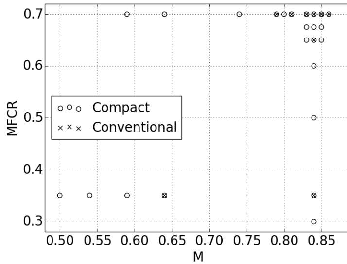
Fig. 6 Conditions measured during the transonic wind tunnel testing in the M-MFCR space. All points were evaluated at \alpha_{nac} = 3.0^\circ and 4.5^\circ
