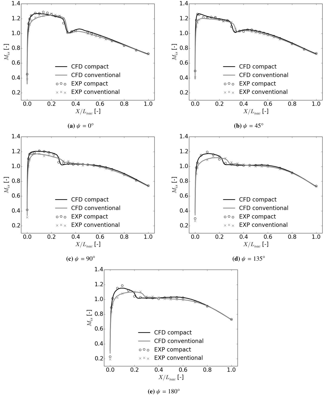
Fig. 7 Isentropic Mach number distribution along the compact nacelle ( L_{nac}/r_{hi} = 3.1 ) and conventional nacelle ( L_{nac}/r_{hi} = 3.6 ) at mid-cruise conditions ( M = 0.85 , MFCR = 0.7 and \alpha_{nac} = 4.5^\circ )
