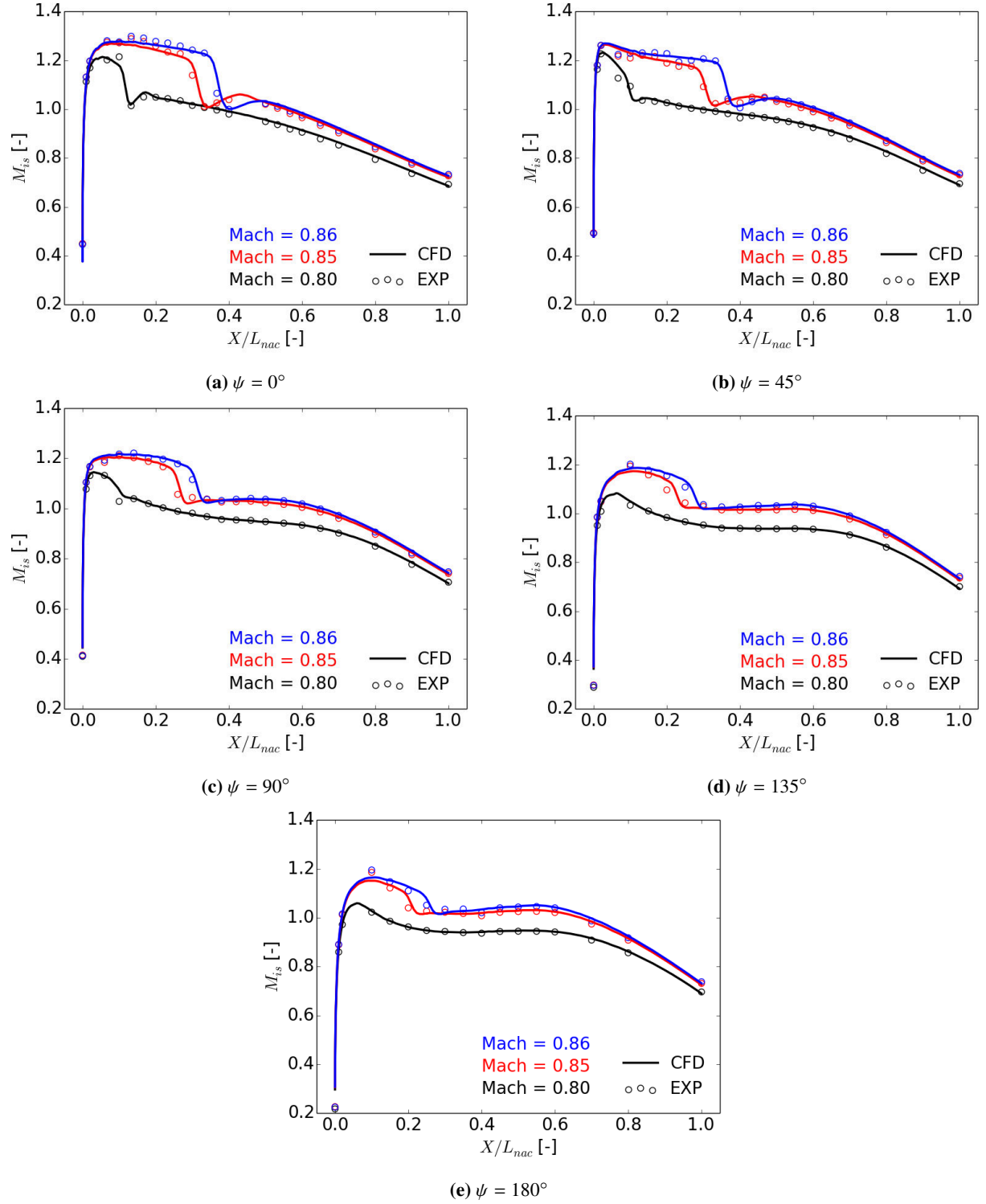
Fig. 11 Isentropic Mach number distribution along the compact nacelle ( L_{nac}/r_{hi} = 3.1 ) as a function of Mach number at fixed MFCR = 0.7 and \alpha_{nac} = 4.5^\circ
