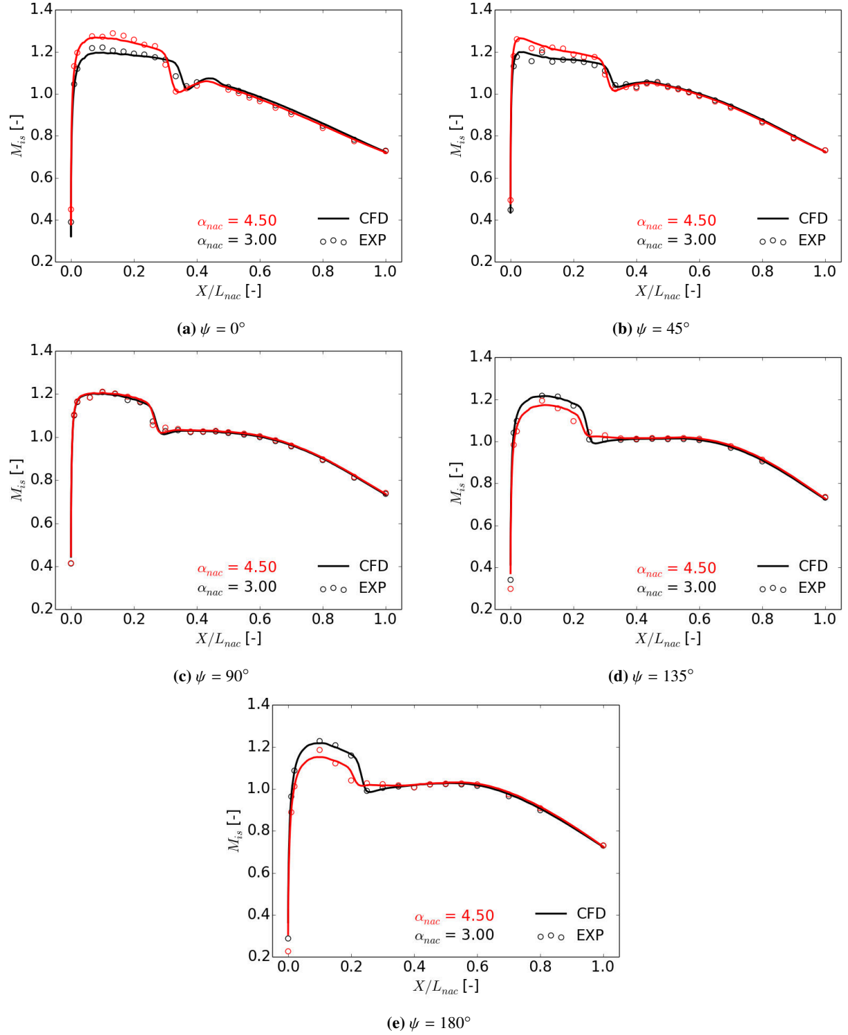
Fig. 14 Isentropic Mach number distribution along the compact nacelle ( L_{nac}/r_{hi} = 3.1 ) as a function of \alpha_{nac} at fixed M = 0.85 and MFCR = 0.7
