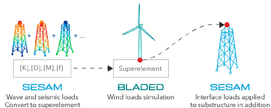
Figure 6. Super-element method [39].
