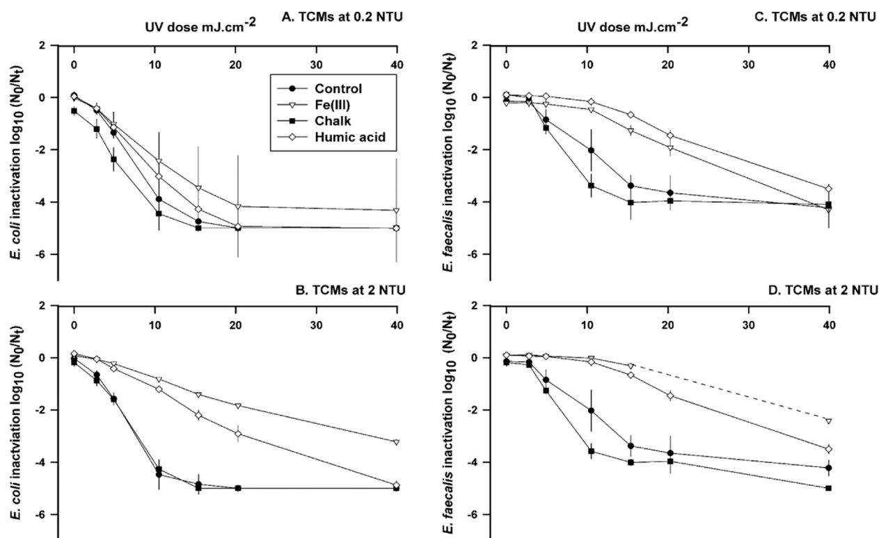
Fig. 3. UV dose on disinfection of bacterial indicators in the presence of TCMs at different turbidity A. E. coli 0.2 NTU, B. E. coli 2 NTU, C. E. faecalis 0.2 NTU and D. E. faecalis 2 NTU. Dashed line indicates missing data point.
