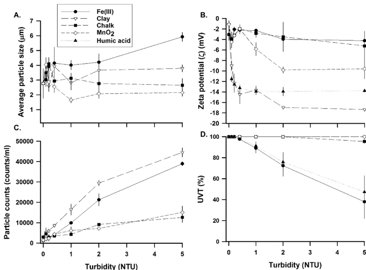
Fig. 1. A. TCM average particle sizes, B. Zeta ( \zeta )-potential of TCMs, C. Particle concentration of TCMs, D. UVT of TCMs at 254 nm. Data represent average \pm 1 standard deviation. Particle size or particle counts were not measured in humic acids.
