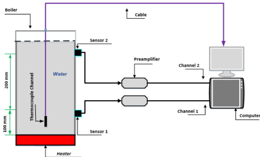
Figure 2: Schematic of experimental arrangement for pool boiling.
