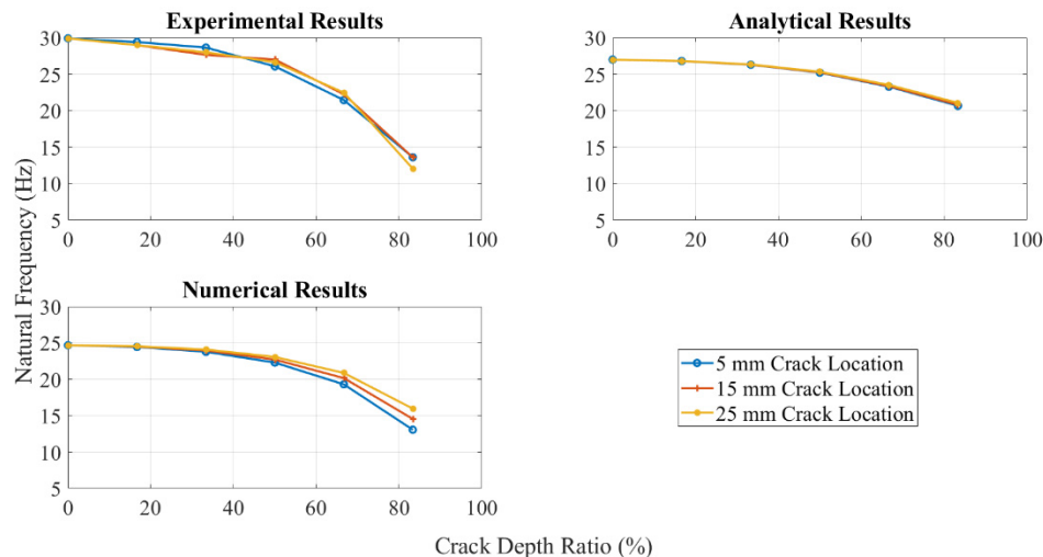
Figure 8. Natural frequency change for crack location by three methods at 25 °C.
