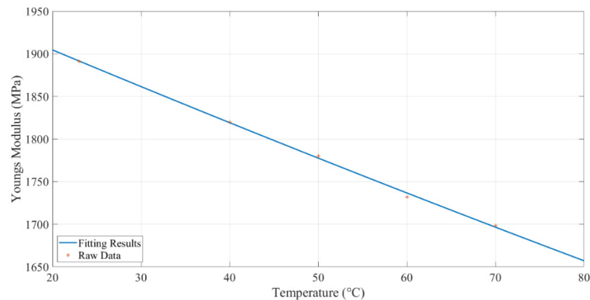
Figure 6. E-modulus curve found based on the natural frequency.
