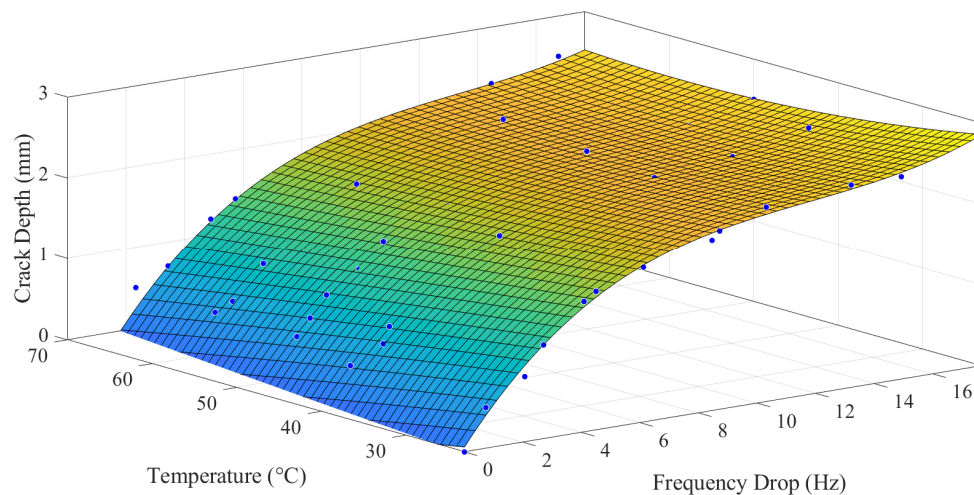
Figure 14. Experimental empirical correlation based on natural frequency for a crack location of 5 mm from the fixed end. Note: The plotted crack depth also includes the initial seeded crack depth value.
