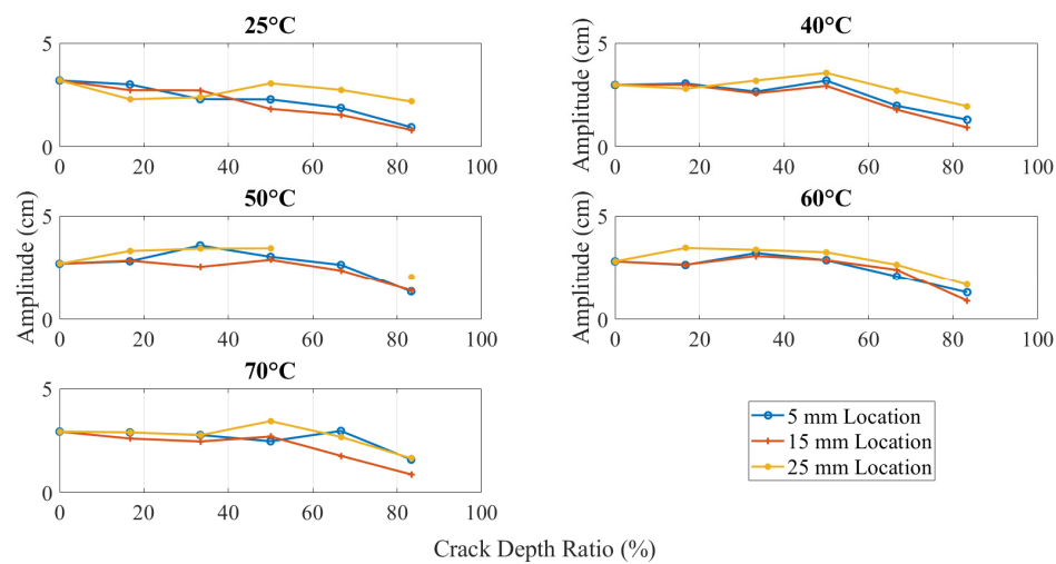
Figure 10. The amplitude of different crack depth beam for the crack at different locations.
