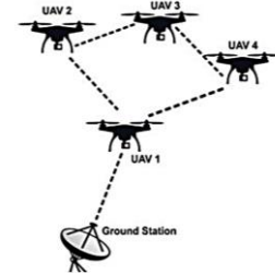
Fig. 7. Flying Ad-hoc Network configuration proposed [20]
