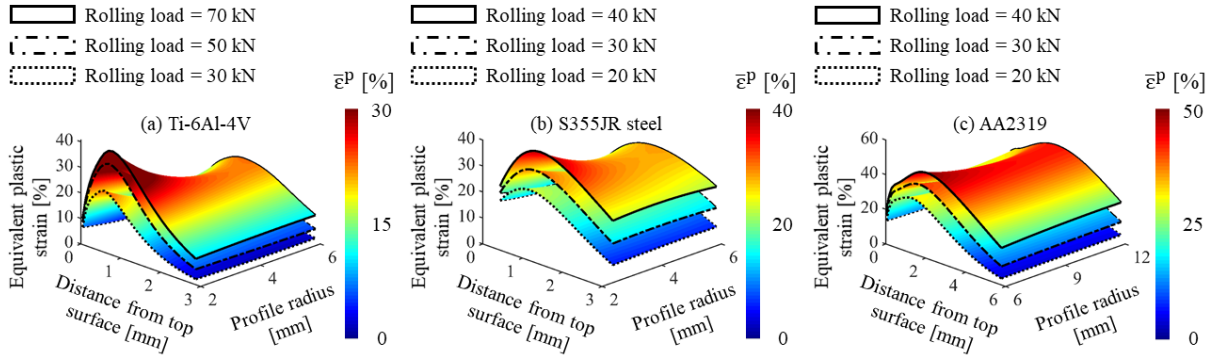
Figure 11: Design curves for equivalent plastic strain as function of rolling profile radius and depth at three different rolling loads for (a) Ti-6Al-4V, (b) S355JR steel and (c) AA2319 walls are shown. Rolling load increases the penetration depth and maximum value of the equivalent plastic strain.
