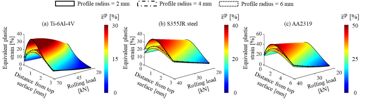
Figure 10: Design curves for equivalent plastic strain as function of rolling load and depth at three different roller profile radii for (a) Ti-6Al-4V, (b) S355JR steel and (c) AA2319 walls are shown.
