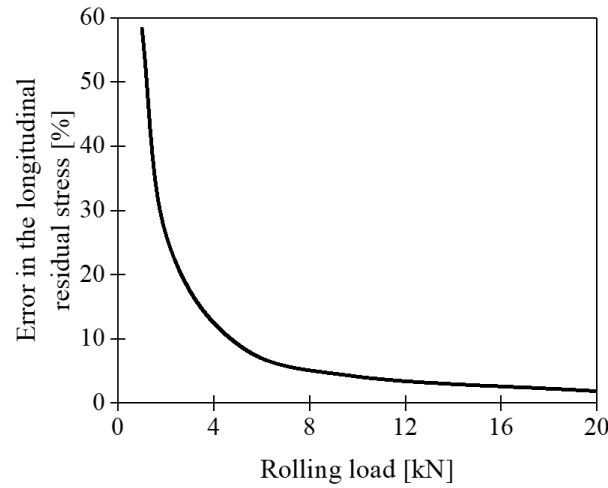
Figure 14: Error in the maximum longitudinal residual stress for different rolling loads in Ti-6Al-4V walls, neglecting the initial residual stresses. The maximum stress in the wall is taken to calculate the error, (\sigma_{\max}^{\text{with int.RS}} - \sigma_{\max}^{\text{without int.RS}}) / \sigma_{\max}^{\text{with int.RS}} . Increasing the rolling load to relevant loads, the effect of the initial state of the wall on the resulting residual stresses becomes negligible.
