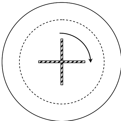
Fig. 4 Cylindrical mixing tank with an MRF boundary surrounding the impeller, from Fluent (2005).
