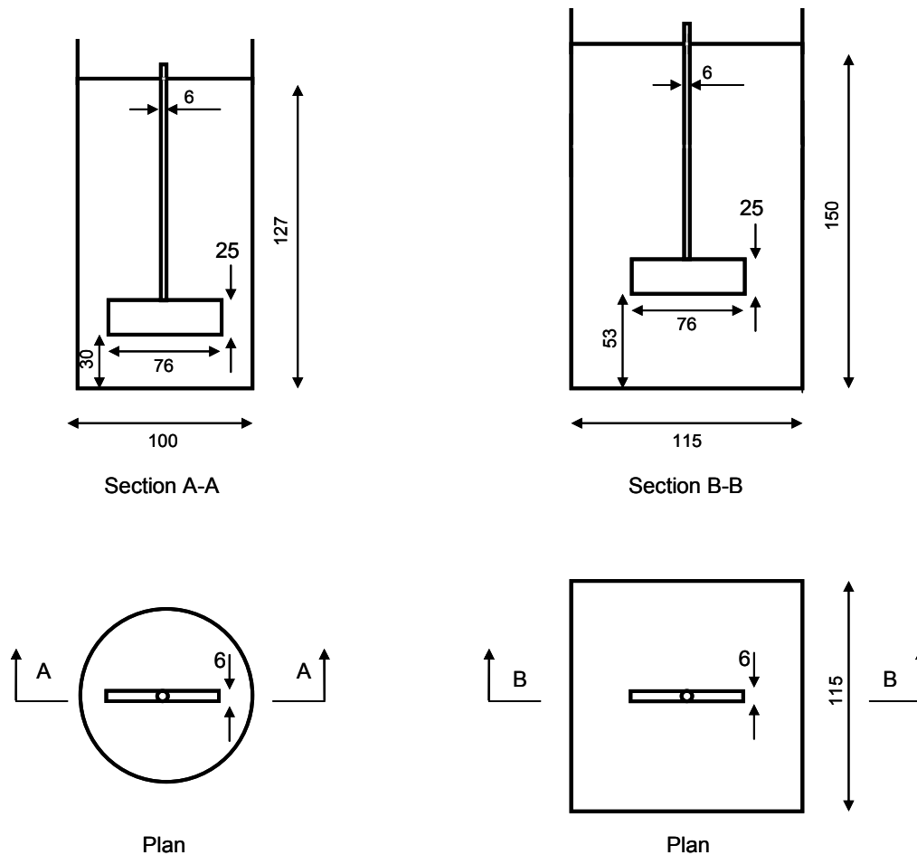
Fig. 2 Typical jar test vessel configurations (not to scale, all dimensions in millimetres).
