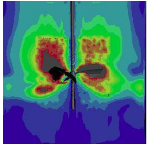
Fig. 5 Distribution of local velocity gradients in a pilot scale mechanical flocculator. Flow rate = 2 \text{ m}^3 \cdot \text{hr}^{-1} , mixing speed = 73 rpm, from Essemiani and de Traversay (2002a).
