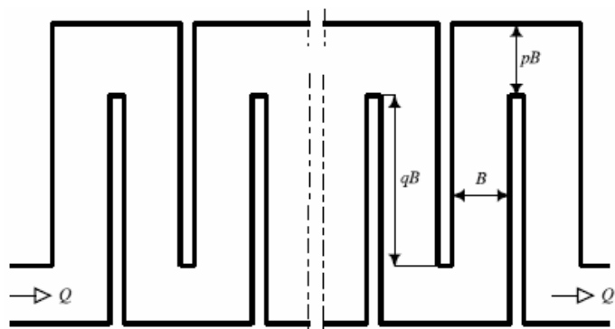
Fig. 1b Schematic diagram of plan view of an hydraulic flocculator, from Haarhoff and Van der Walt (2001).
