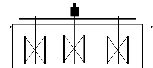
Fig. 1a Schematic diagram of sectional view of a mechanical flocculator.
