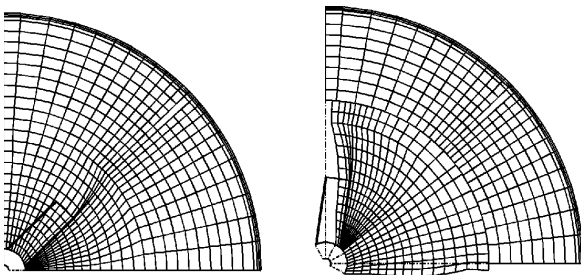
Fig. 3 Sliding mesh in two orientations, shown in 2D, from Marshall and Bakker (2004).
