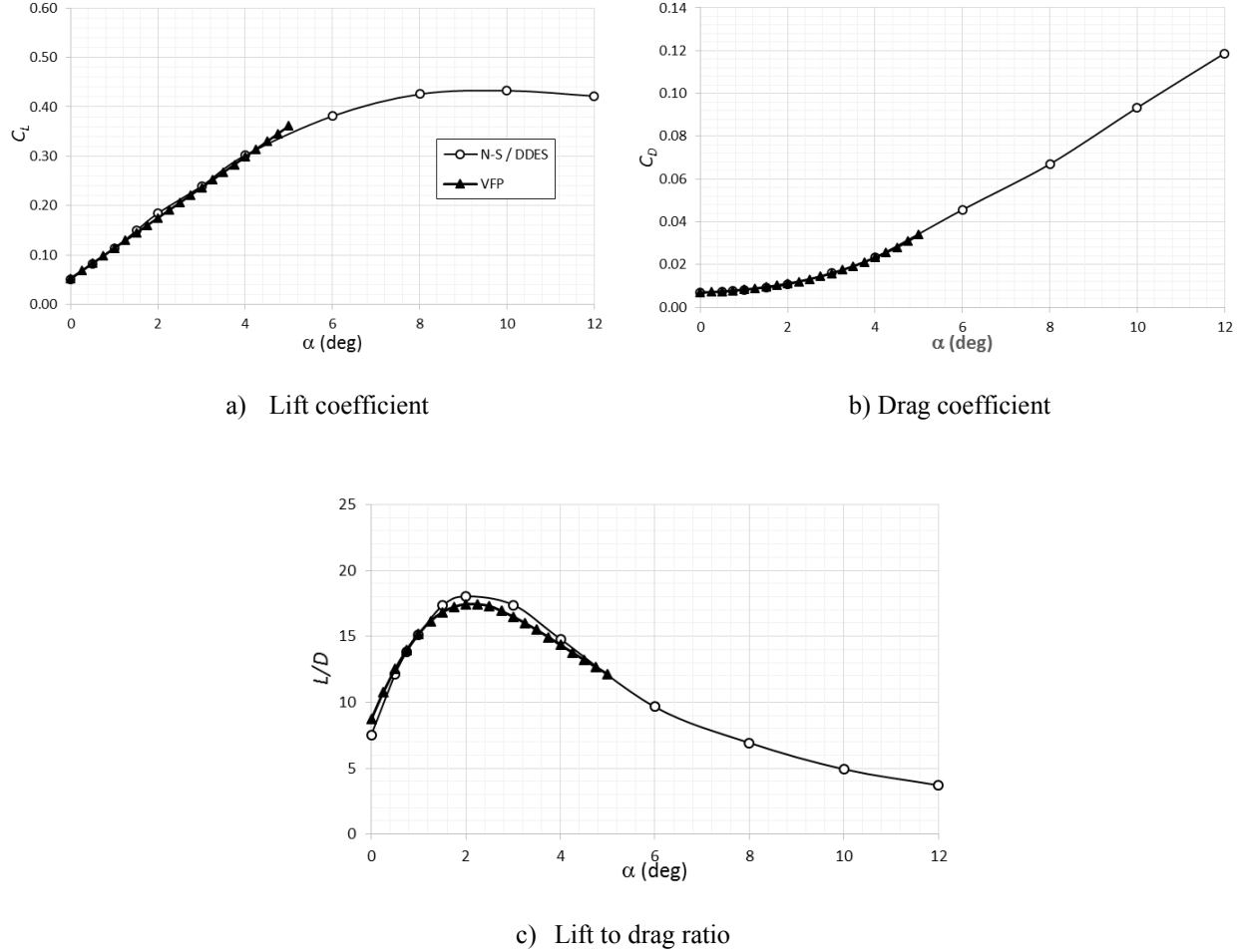
Fig. 8. Comparison of predicted force characteristics, M=0.80 , Re=7.4 \times 10^8 .
