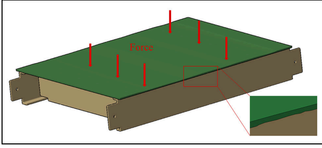
Figure 3. Mating surface of two non-ideal components.
