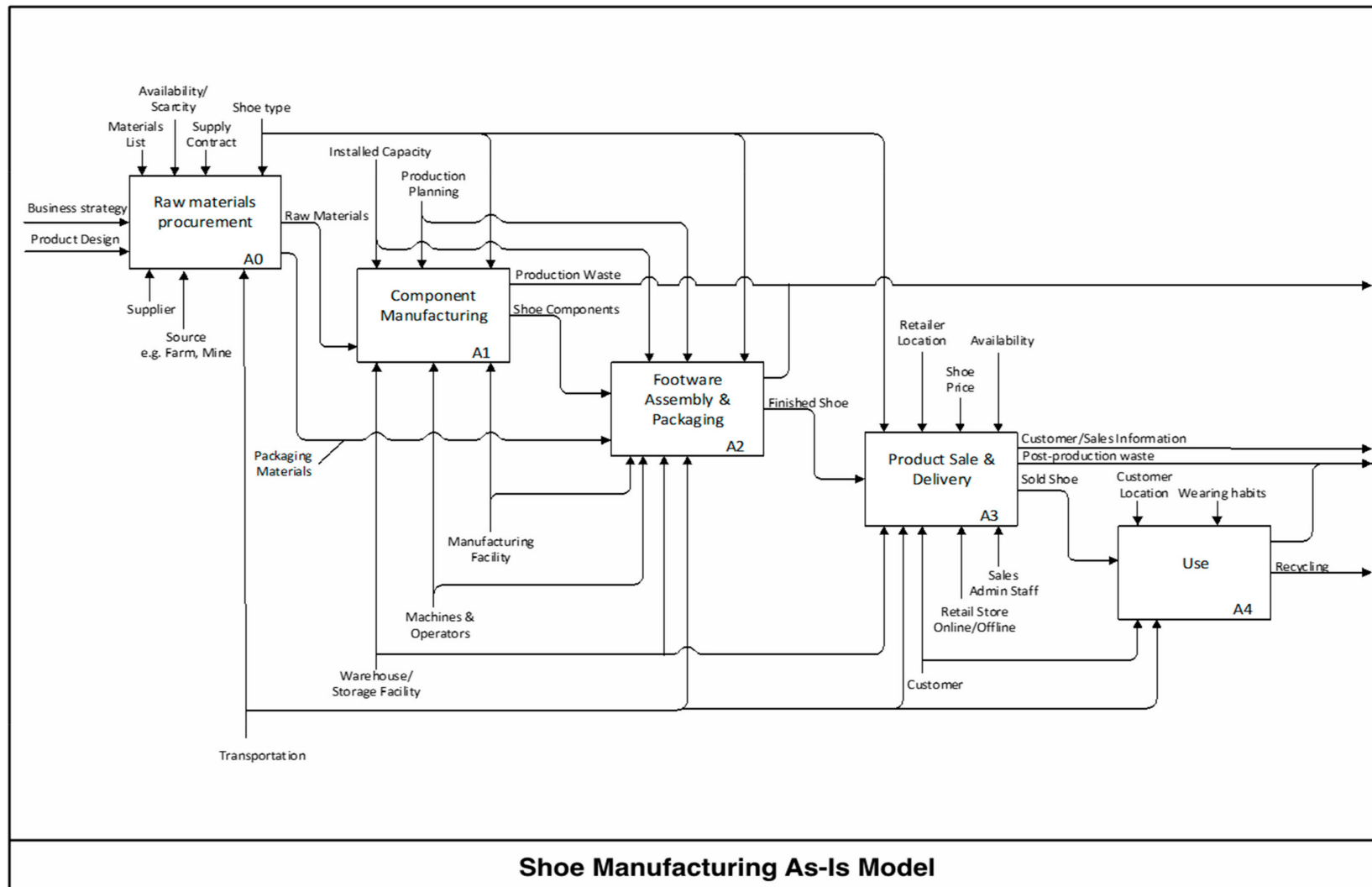
Figure 4. Shoe Manufacturing As-Is Model.
