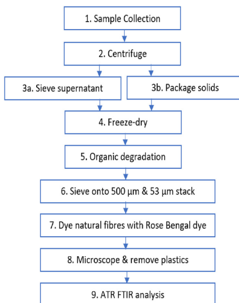
Fig. 3. Flow chart of the sequential steps for the analysis of microplastics in wastewater sludge.
