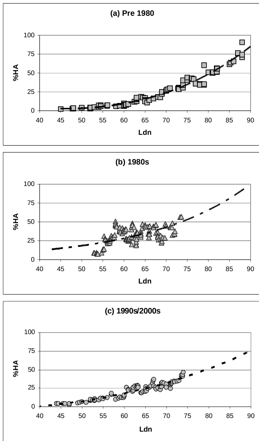
Figure 5. Fidell & Silvati %HA data, time groups, 7-point moving average, fitted lines (a) and (c) cubic, (b) exponential
