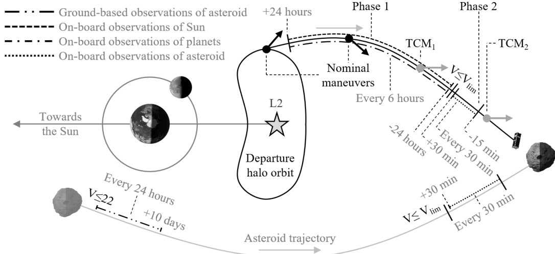
Fig. 4. Diagram of mission profile, including on-board navigation and guidance strategies.
