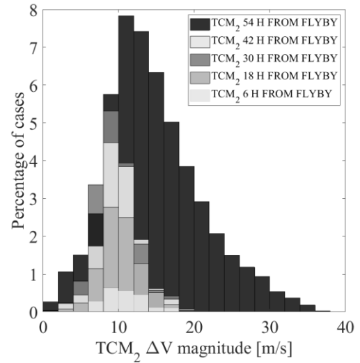
Fig. 11. Histogram of actually-executed TCM 2 \Delta V magnitudes (asteroid 2017 XC62, and 2-m/s discretization bins).
