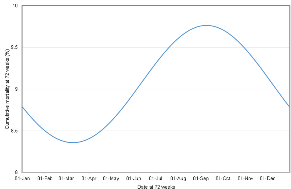
Fig 2. Predicted CM for a free range flock reaching 72 weeks at different times of year (modelled from 2,848 flocks, on 1,649 farms, from six studies).
