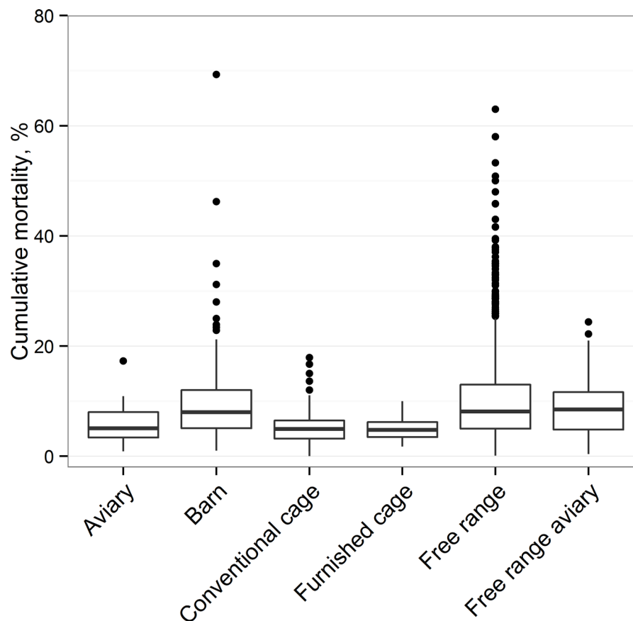
Fig 1. Box plots for mortality in each housing system between 60 and 80 weeks of age using the full data set from 10 studies (3,851 flocks).
