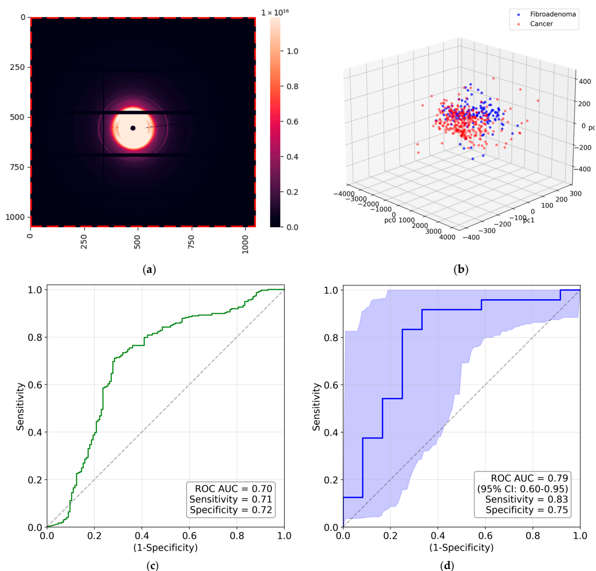
Figure 3. (a) SAXS image with excluded triglyceride peak; (b) the PCA-transformed data within the 3D PC space. Each PCA point corresponds to a single diffraction measurement; (c) measurement-based ROC curve for collagen contribution to synchrotron SAXS images; (d) patient-based ROC curve with the 95% confidence interval for collagen contribution to synchrotron SAXS images.
