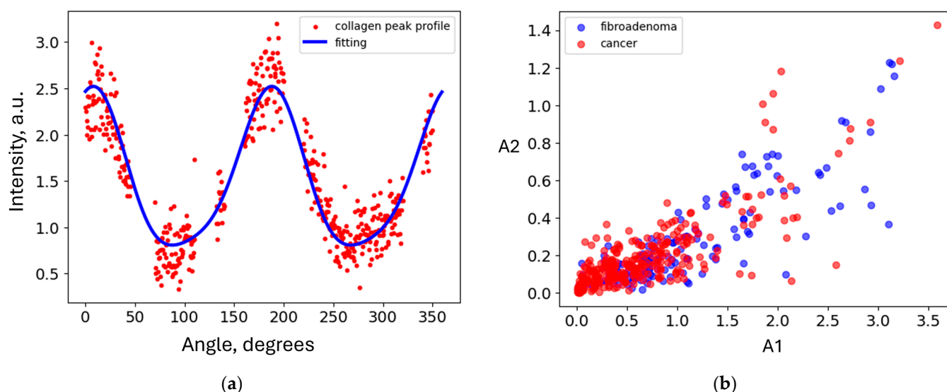
Figure 2. (a) The anisotropy of the signal at the 3rd order collagen peak at q = 0.3 nm -1 . The blue line indicates the fitting based on two sinusoidal functions. (b) Measurements of cancerous (red) and fibroadenoma (blue) samples in the space of the two coefficients of the sinusoidal functions.
