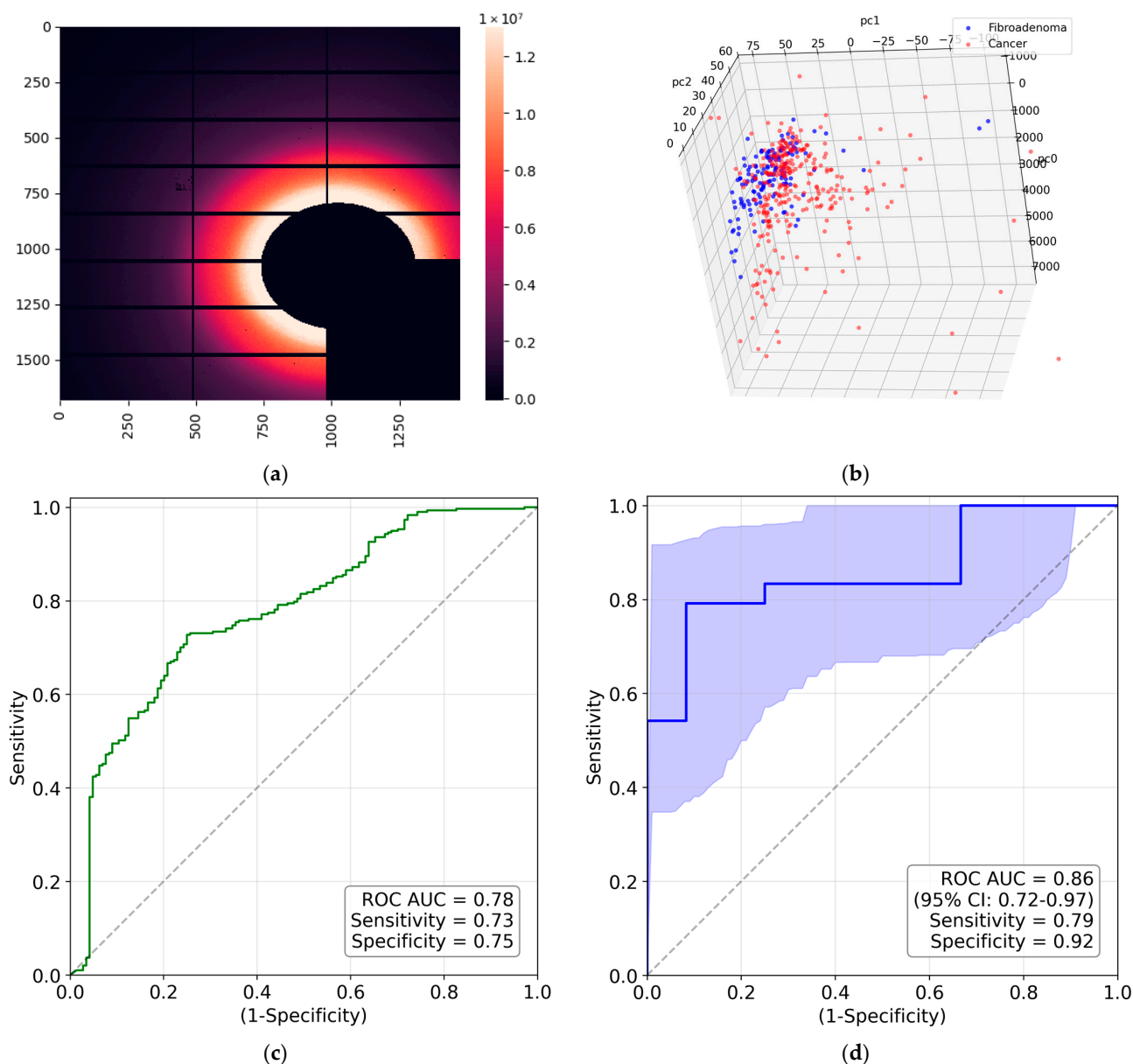
Figure 4. (a) WAXS image with excluded lipid maximum; (b) the PCA-transformed data within the 3D PC space. Each PCA point corresponds to a single diffraction measurement; (c) measurement-based ROC curve for water contribution to synchrotron WAXS images; (d) patient-based ROC curve with the 95% confidence interval for water contribution to synchrotron WAXS images.
