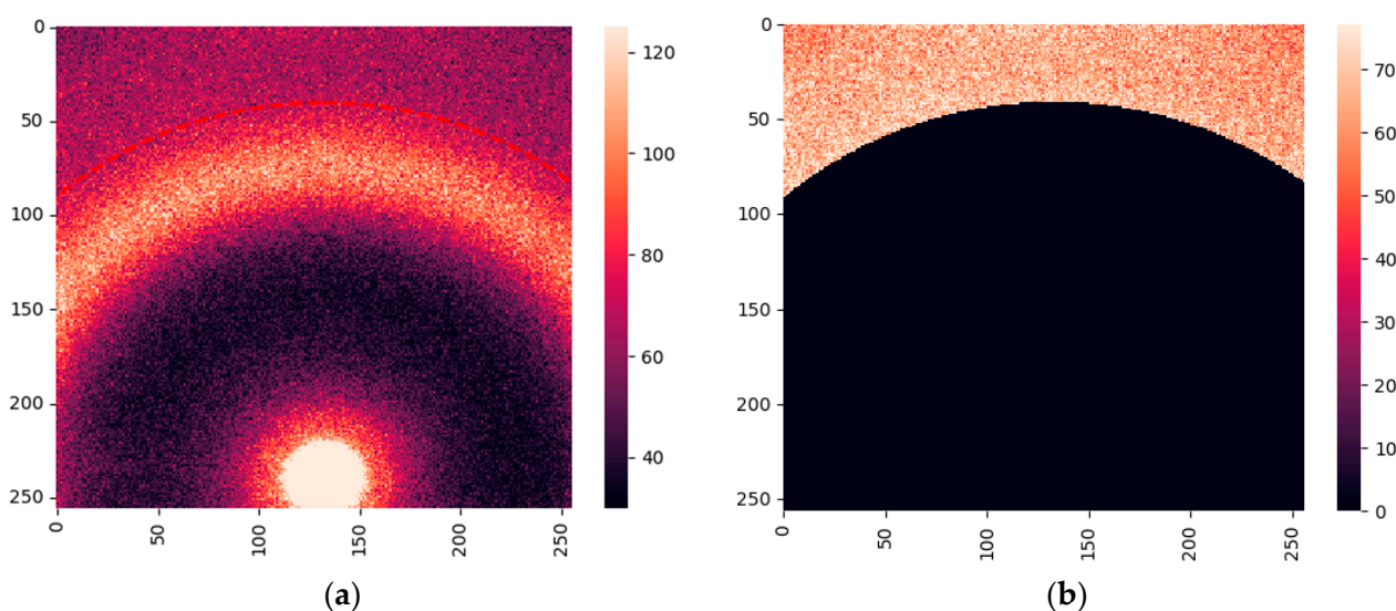
Figure 5. X-ray scattering images obtained at a laboratory diffractometer. Numbers indicate the position of the pixels on the detector. (a) Full image; (b) image with only water contribution. The red dashed line indicates the extracted boundary.
