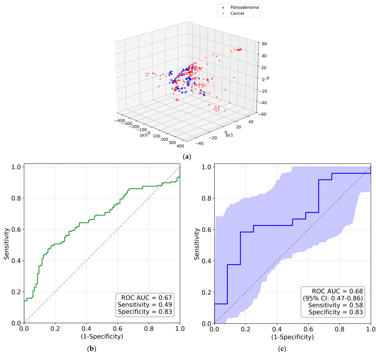
Figure 6. (a) The PCA-transformed data within the 3D PC space; (b) measurement-based ROC curve for water contribution to laboratory WAXS images; (c) patient-based ROC curve with the 95% confidence interval for water contribution to laboratory WAXS images.
