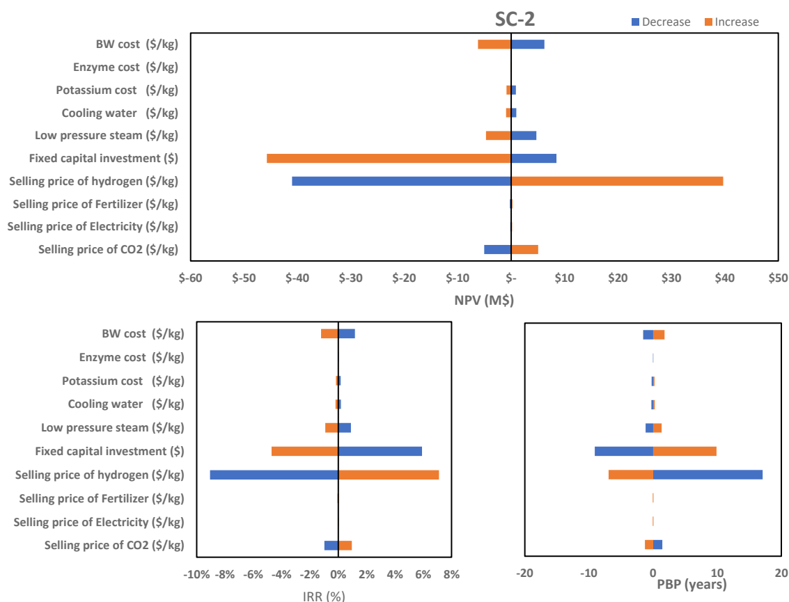
Fig. 5. Sensitivity analysis for different scenarios: (a) SC-1; (b) SC-2.
