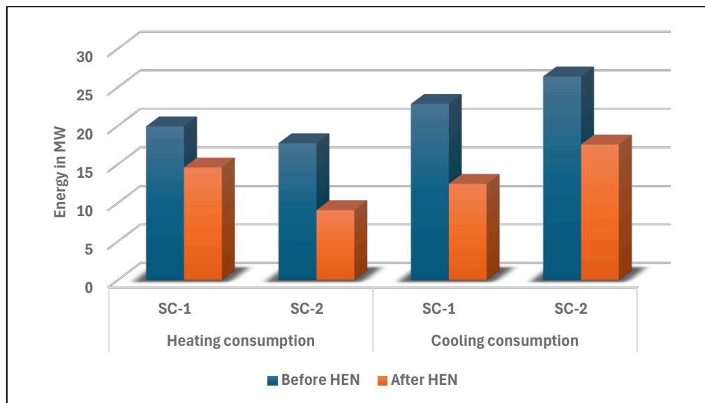
Fig. 3. Energy (heating and cooling) requirements before and after integration.
