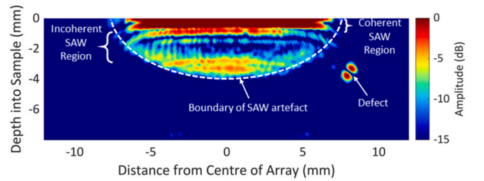
Fig. 3. TFM image using transverse wave velocity showing the various regions of SAW artefact from a Ti-6Al-4V sample. The image was acquired using a 71 element LIPA of 14 mm aperture.
