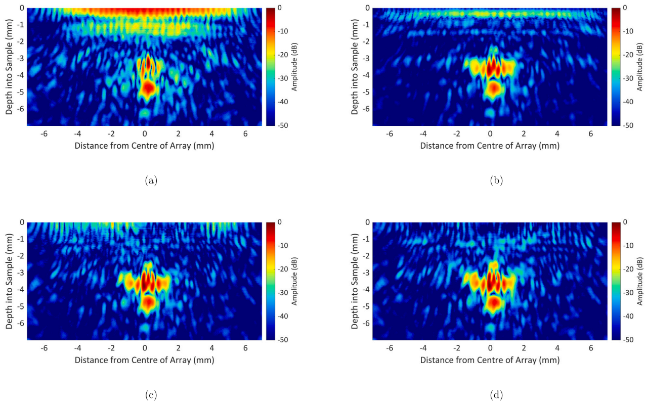
Fig. 12. TFM ultrasonic images obtained by implementing PCI after (a) amplitude thresholding, (b) f - k filtering, (c) mean waveform subtraction, (d) principal component subtraction.
