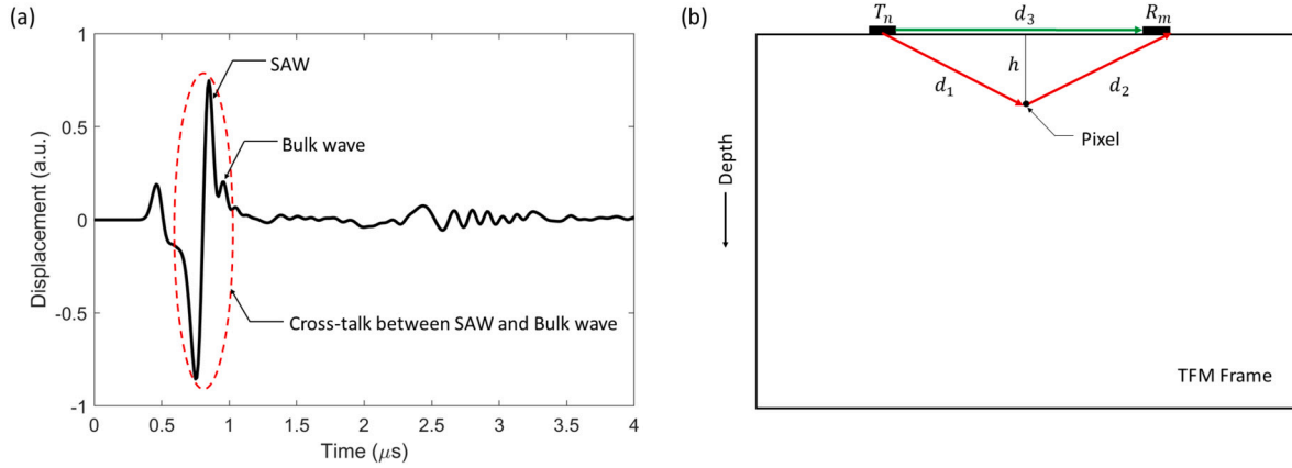
Fig. 2. (a) Finite element simulation generated ultrasonic signal showing the temporal SAW crosstalk phenomenon, (b) schematic demonstrating the principle of temporal SAW crosstalk.
