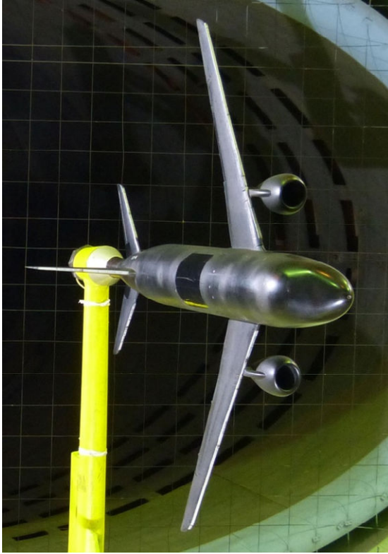
Fig.1. Fully iced aircraft model installed on the tail support strut in the wind tunnel test section.
