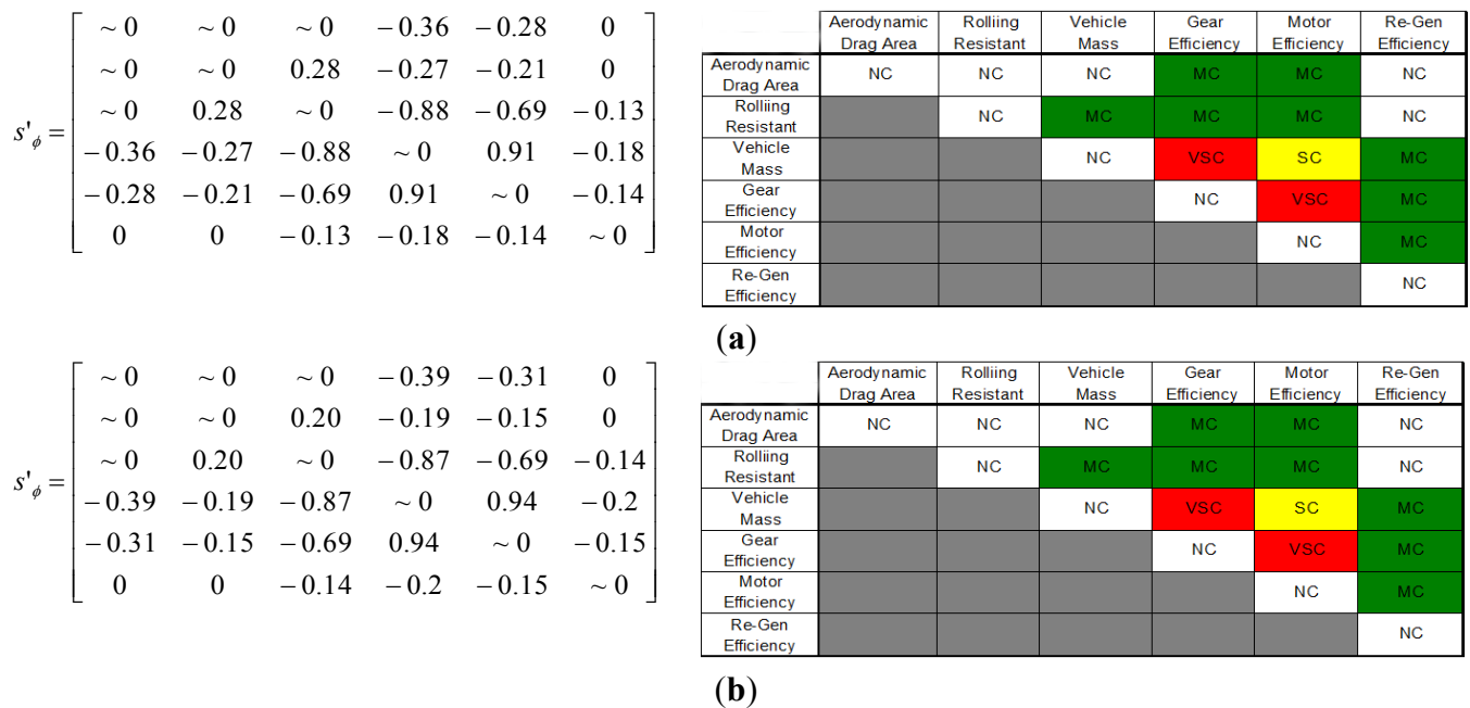
Figure 5. Second-order sensitivity analysis for the nominal vehicle parameters. (a) NEDC and (b) Artemis.
