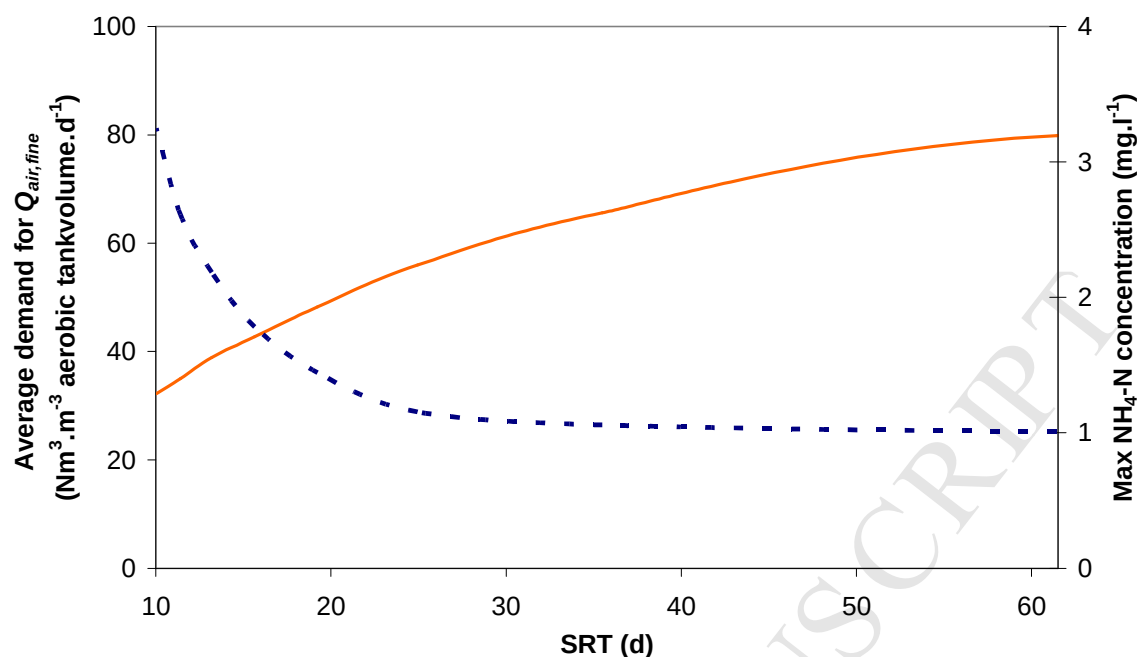
Figure 6: Influence of wastage rate on the total demand for biology aeration ( Q_{air,fine} ) and the maximum occurring effluent \text{NH}_4\text{-N} concentration during the 35-day simulation ( Q_{air,coarse} = 42 \text{ Nm}^3 \cdot \text{h}^{-1} ; DO setpoint = 1.25 \text{ mg} \cdot \text{l}^{-1} ; recirculation flow = 108 \text{ m}^3 \cdot \text{d}^{-1} )
