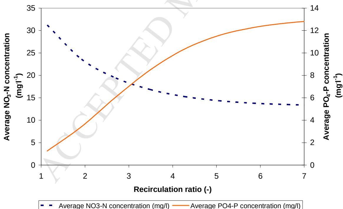
Figure 7: Influence of recirculation flow rate on the average effluent \text{NO}_3\text{-N} and \text{PO}_4\text{-P} concentrations during the 35-day simulation ( Q_{air,coarse} = 42 \text{ Nm}^3 \cdot \text{h}^{-1} ; DO setpoint = 1.25 \text{ mg} \cdot \text{l}^{-1} )
