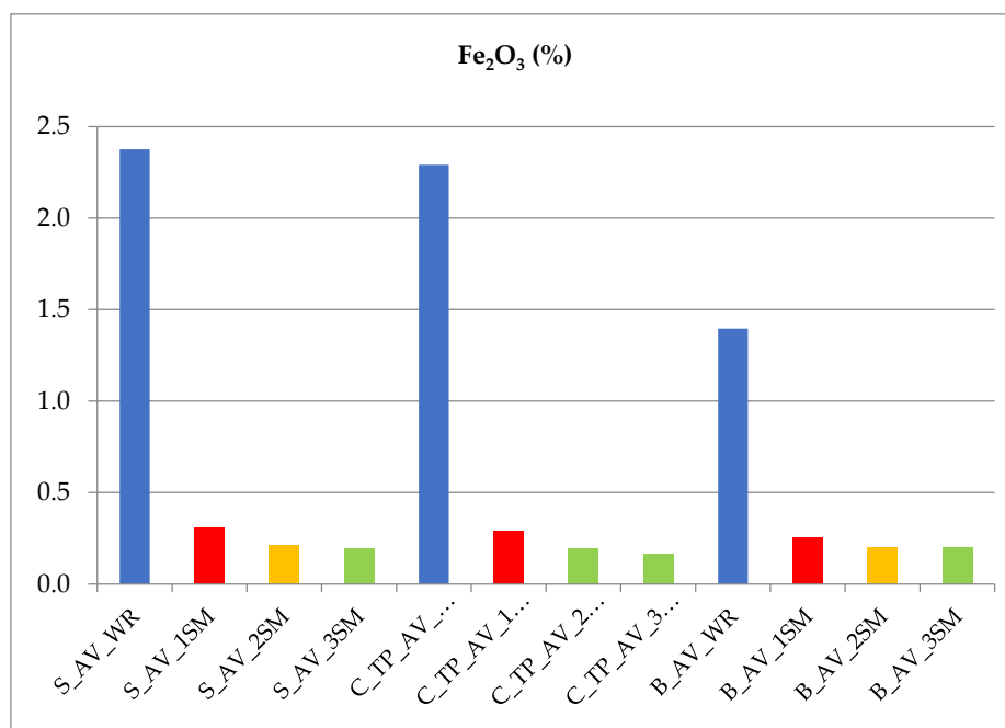
Figure 8. Concentration of Fe 2 O 3 tot in the S-Sengio, C-Ciana-Tane Pilastretto and B-Braghini EW facilities (all samples; values in wt %). blue: WR; red: nonmagnetic fraction >0.2%; orange: nonmagnetic fraction just above 0.2%; green: nonmagnetic fraction <0.2%.
