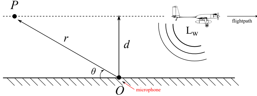
Fig. 5 Diagram of typical flyover procedure for obtaining NPD data. Adapted from [6].
