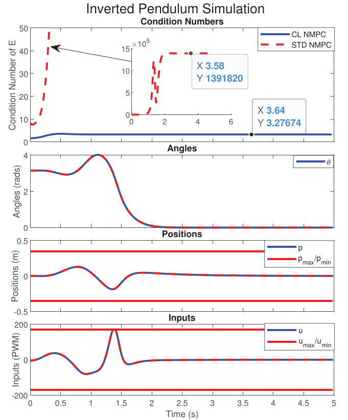
FIGURE 2 Example numerical conditioning using double precision with initial condition x_0 = [0, 0, 0, \pi]^T , N_p = 75 . STD and CL refer to the standard and proposed closed loop solution, respectively
