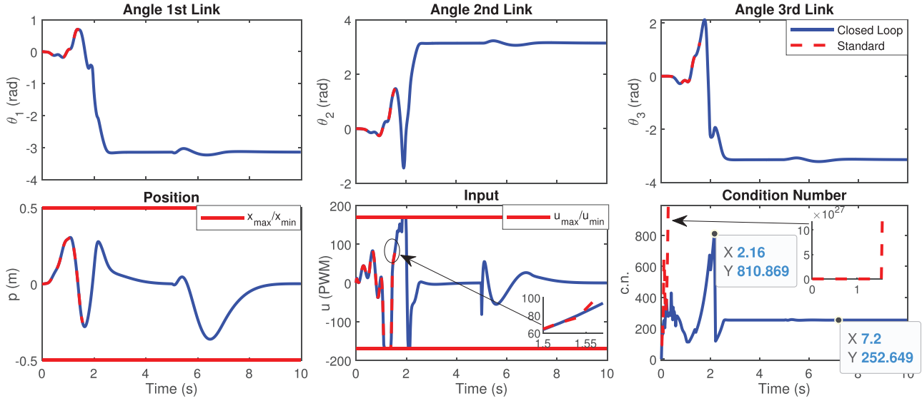
FIGURE 5 Triple inverted pendulum swing up and stabilisation simulation with disturbance of x_k = x_k + [0, 0, 0, 0.1, 0, 0, 0, 0]^T injected at t = 5 (s). The maximum and steady state conditioning numbers are shown in the lower-right figure for reference
