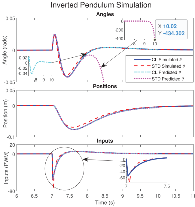
FIGURE 3 Disturbance response - prediction and simulated comparison for N_p = 150 when using Matlab “inv(A)” function. Disturbance of x_k = x_k + [0, 0.5, 0, 0]^T was injected at t = 7 (s). STD and CL refer to the standard and the proposed closed loop solutions, respectively
