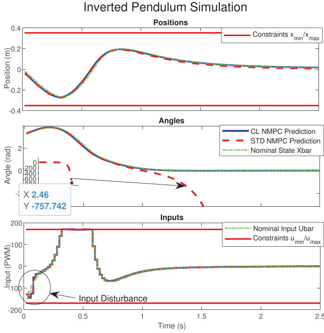
FIGURE 4 Example “free-response” predictions comparison with a random input disturbance during swing up with N_p = 150 . STD and CL refer to the standard and closed loop solutions, respectively
