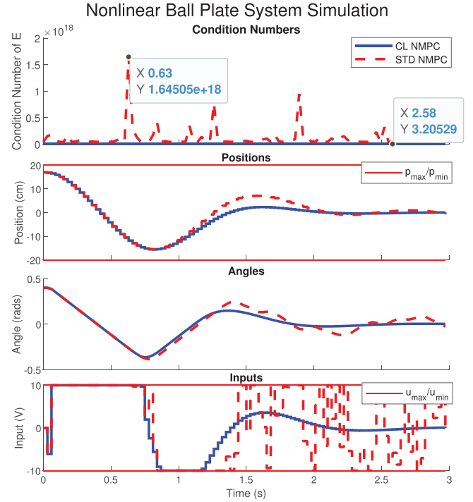
FIGURE 1 Nonlinear ball plate system simulation with initial condition x_0 = [17, 0, 0.4, 0]^T and prediction horizon of N_p = 20 . CL and STD represent the proposed closed loop and the standard approach, respectively
