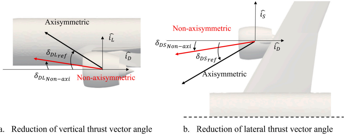
Fig. 11. Reduction of (a) vertical and (b) lateral thrust vector angles produced by non-axisymmetric exhausts.
