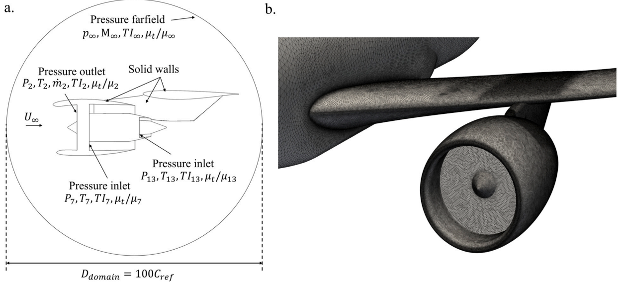
Fig. 5. (a) Schematic of the computational domain and boundary conditions and (b) surface mesh.
