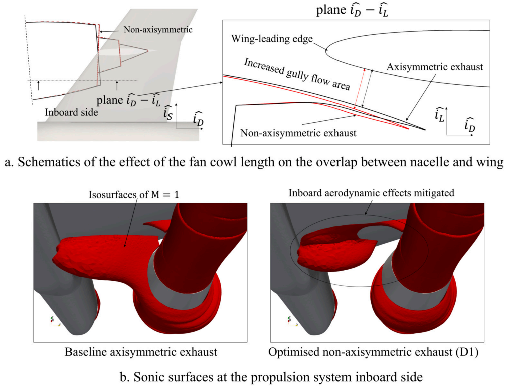
Fig. 17. Effect of non-axisymmetric exhausts on the inboard aerodynamics. (a) Schematics of the overlap between nacelle and wing and (b) rear views of axisymmetric (left) and non-axisymmetric (right, D1) exhausts. Red isosurfaces are of M = 1 .
