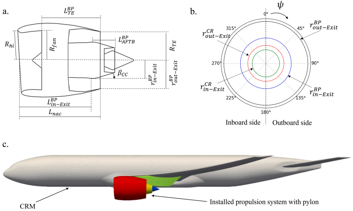
Fig. 1. Baseline propulsion system configuration with (a) side and (b) nozzle views. (c) Schematic of a propulsion system installed with the CRM.
