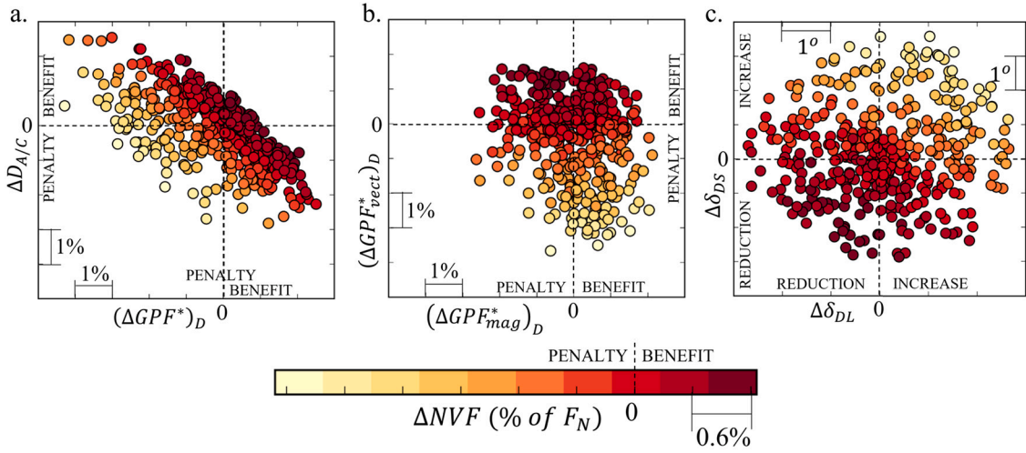
Fig. 10. Summary of the design space exploration results with splits of (a) (\Delta GPF^*)_D and \Delta D_{A/C} , (b) (\Delta GPF^*_{vec})_D and (\Delta GPF^*_{mag})_D , (c) \Delta \delta_{DL} and \Delta \delta_{DS} .
