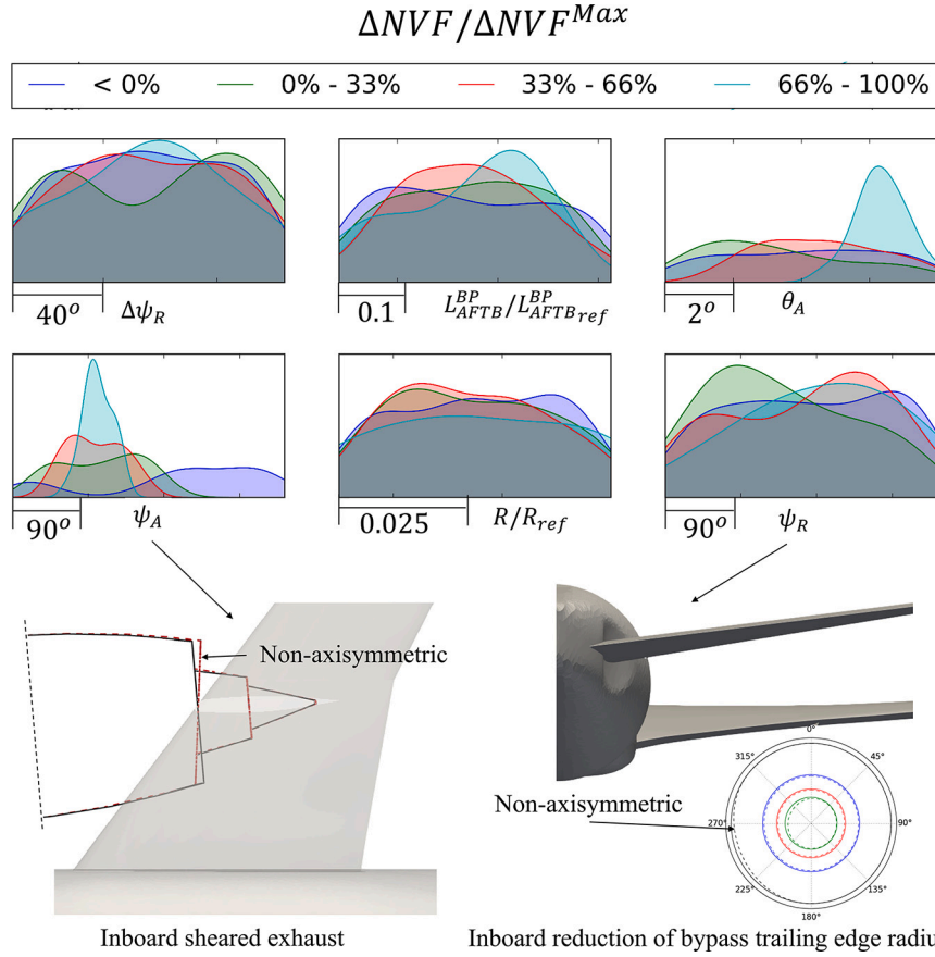
Fig. 12. Histograms of the distribution of designs in the design space. The database is classified in bands of different levels of \Delta NVF .
