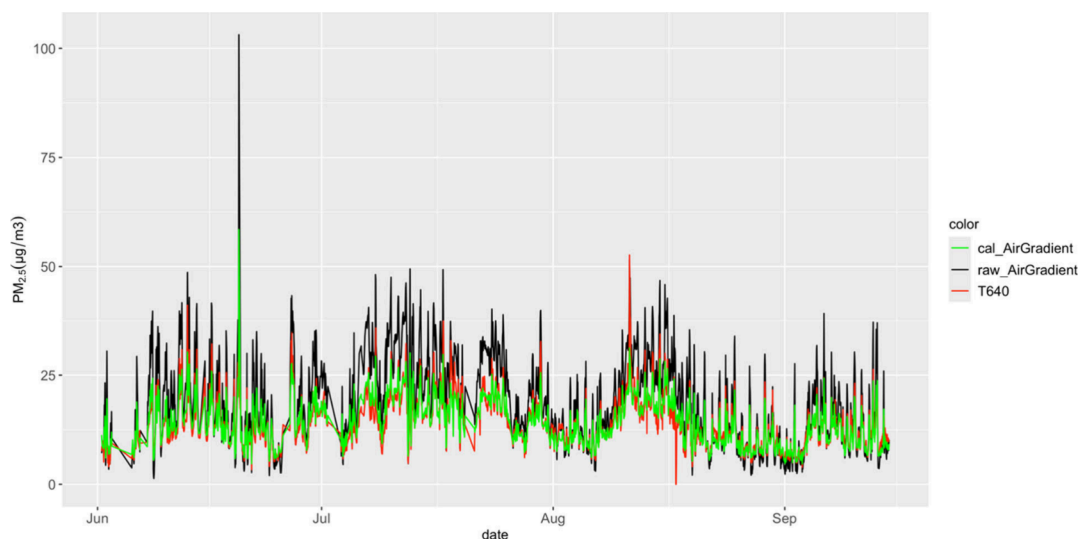
Figure 4. Time series plot for PM 2.5 showing AirGradient raw (black), calibrated (green), and T640 (red) on hourly data sets.
