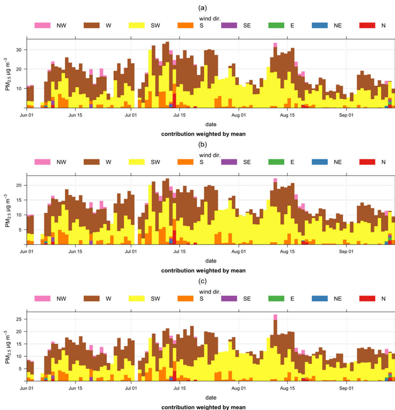
Figure 9. Time series plot for \text{PM}_{2.5} as a function of wind direction raw AirGradient (a), calibrated AirGradient (b), and T640 (c) on hourly data sets.
