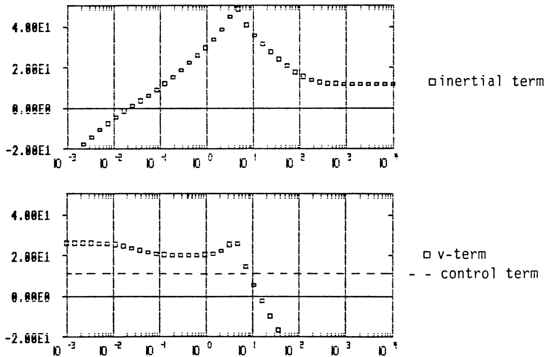
Fig. 4.3 Bode plot of the Y-equation terms
