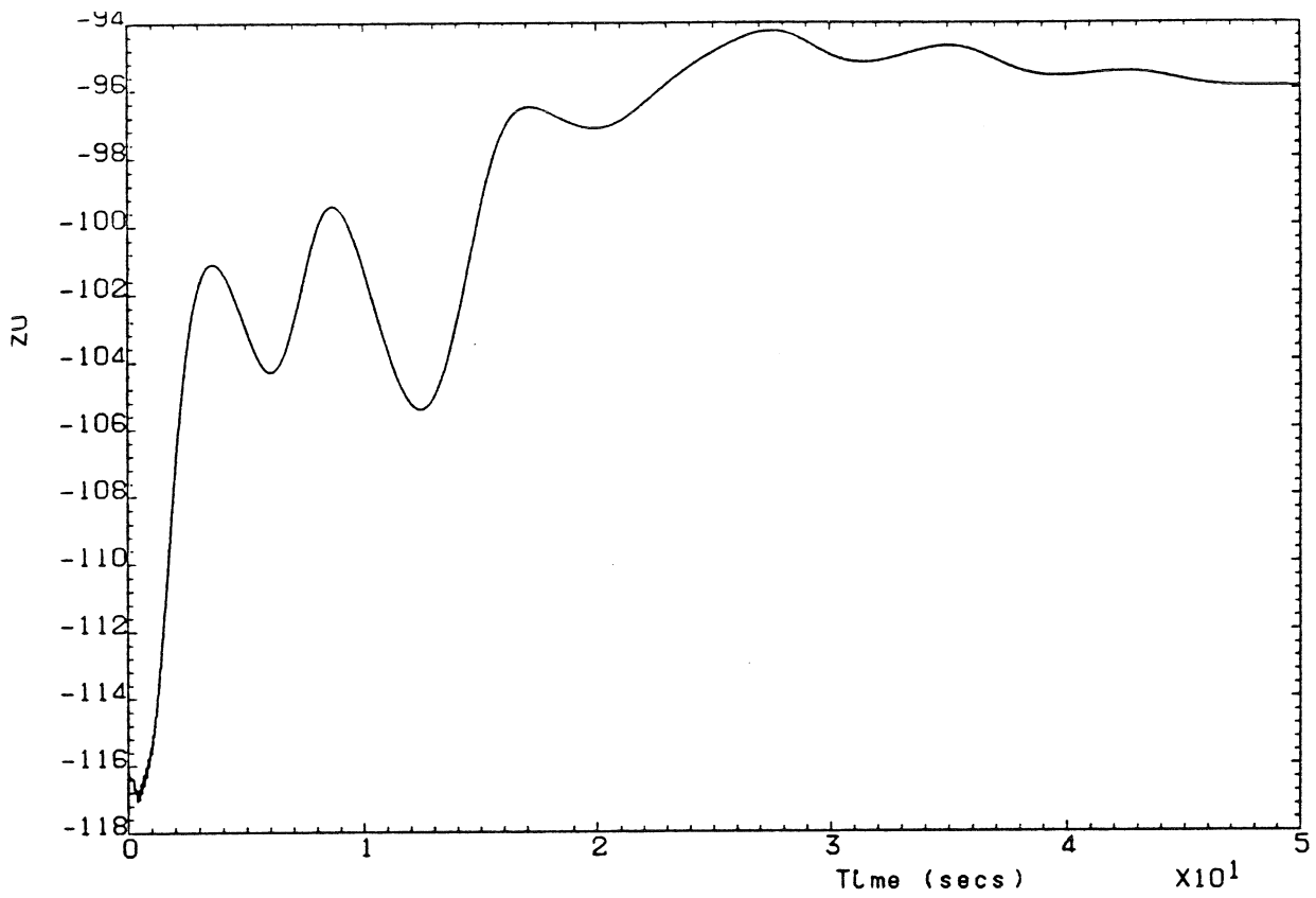
Fig. PI.1-4 z_u estimate (square wave input)
