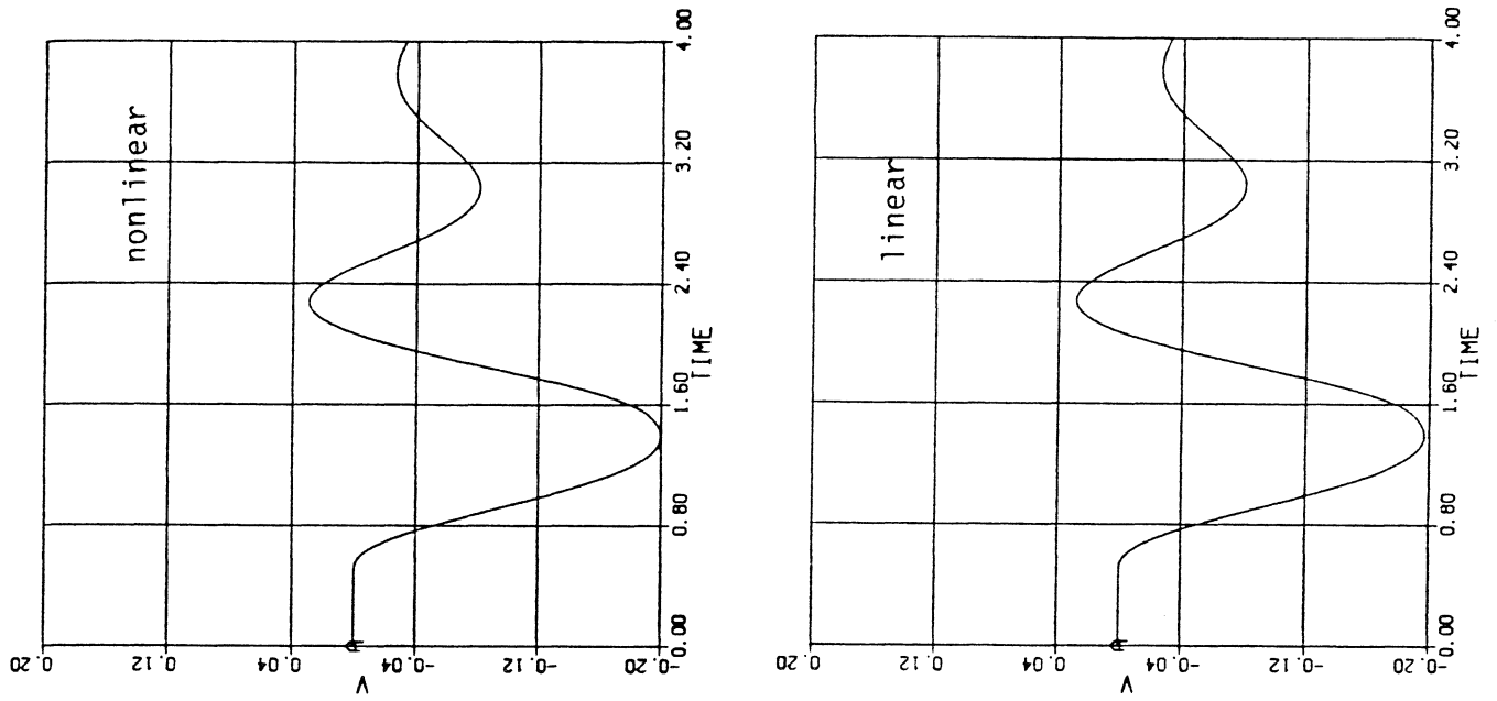
Fig. 3.12 v response to aileron deflection
