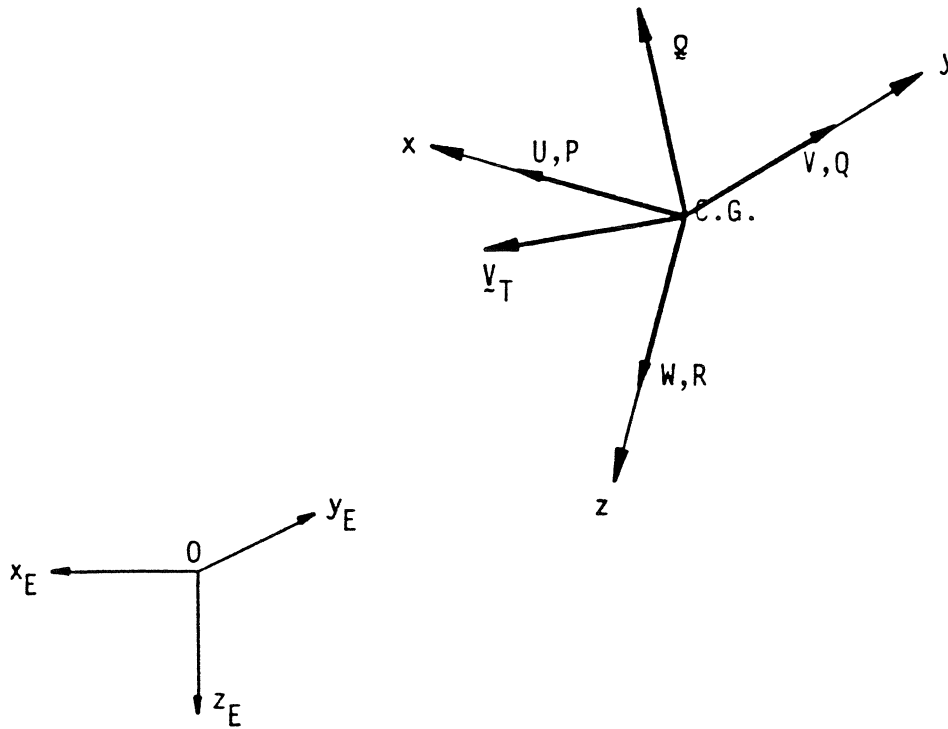
Fig. 1.3 Aircraft movement w.r.t. earth
