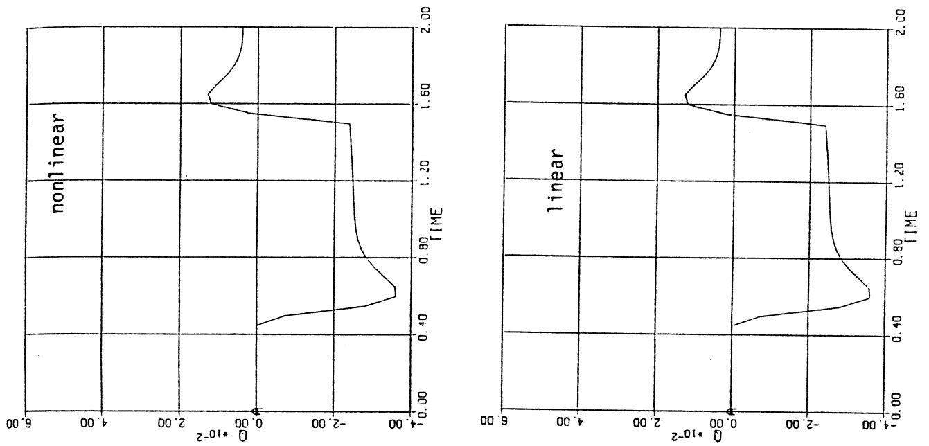
Fig. 3.5 q response to elevator deflection
