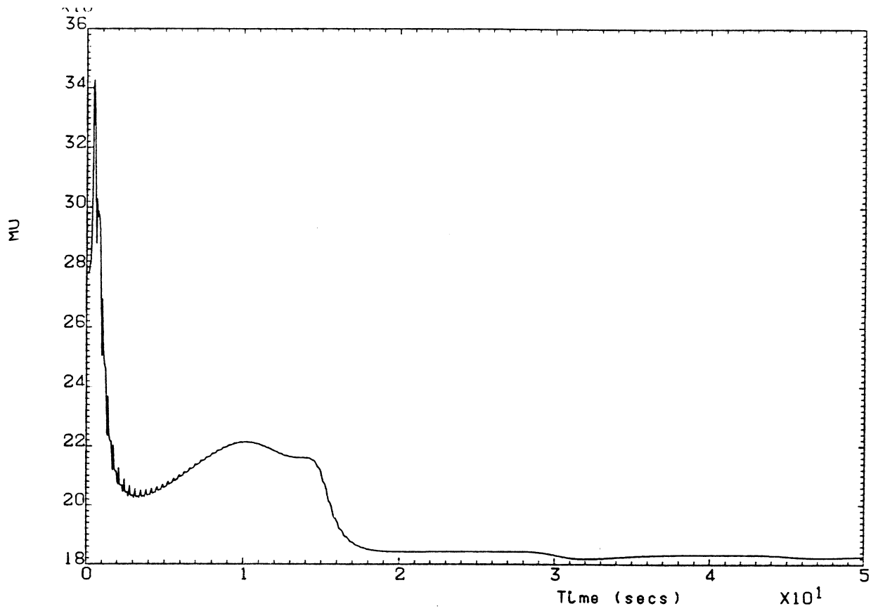
Fig. PI.1-14 m_u estimate (multistep input)
