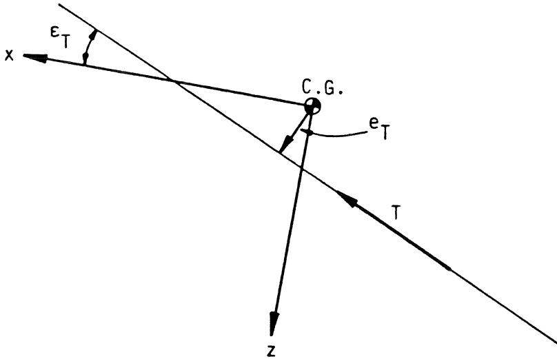
Fig. 1.5 Thrust configuration
