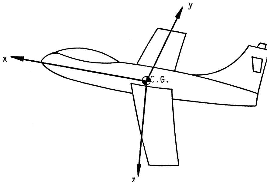
Fig. 1.1 Body-fixed Axes
