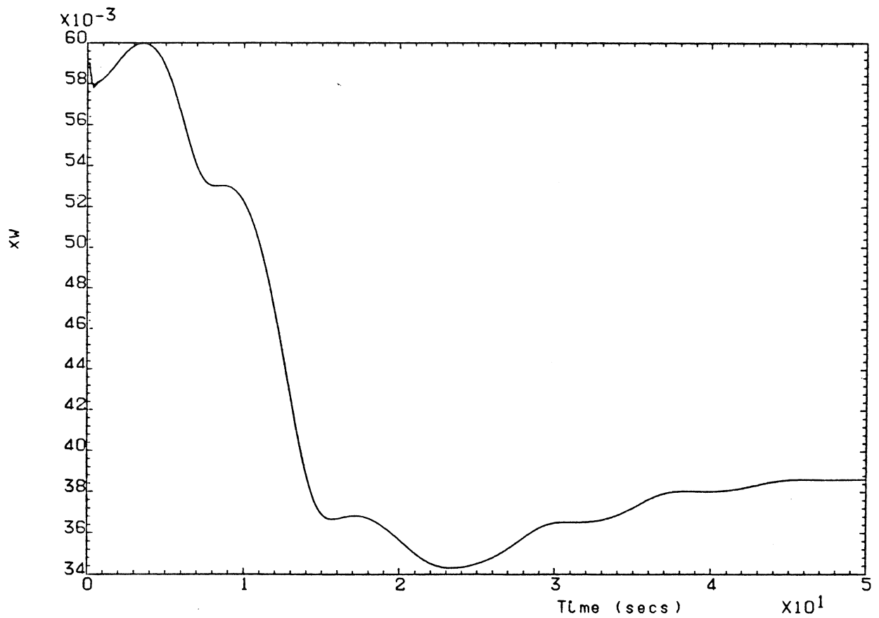
Fig. PI.1-3 x_w estimate (square wave input)
