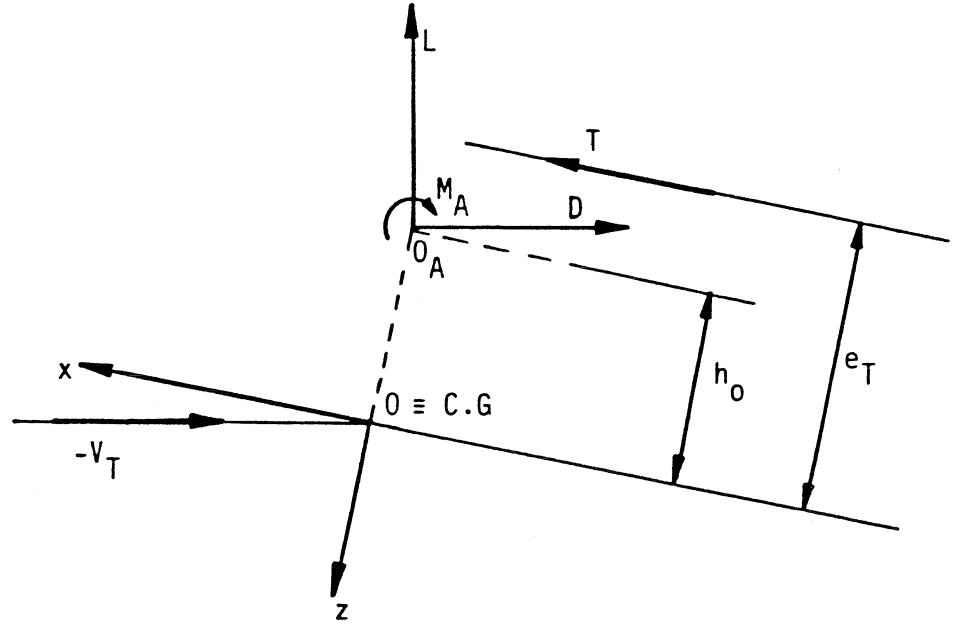
Fig. 3.2 Pitching moment reference point
