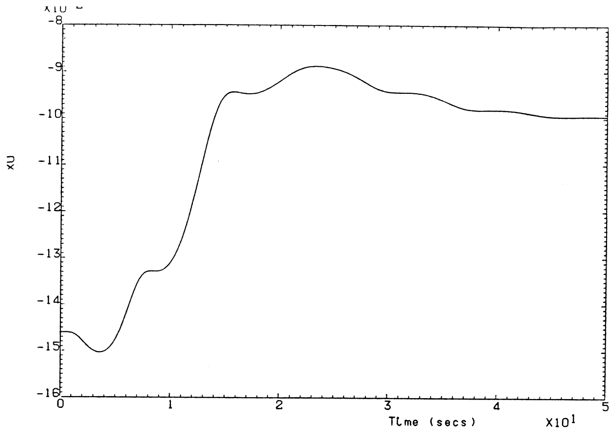
Fig. PI.1-2 x_u estimate (square wave input)
