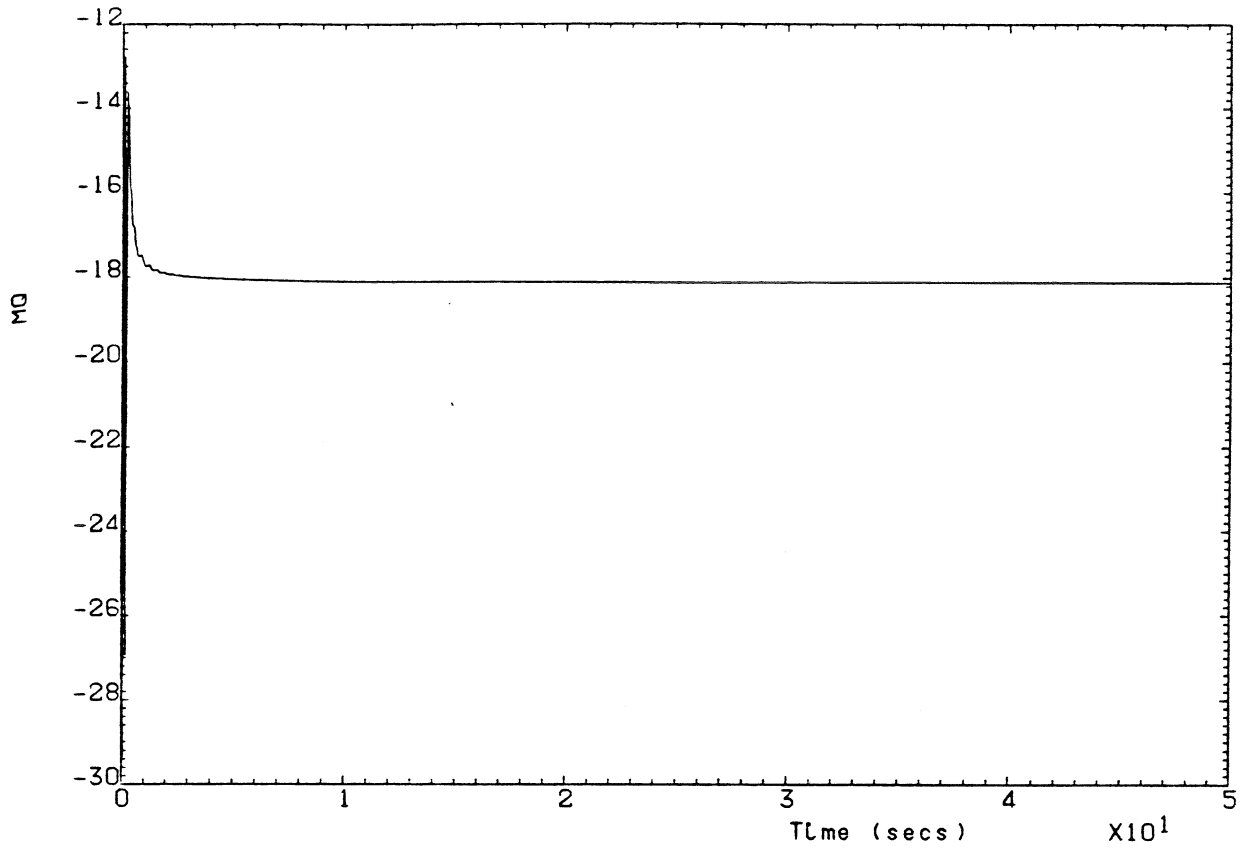
Fig. PI.1-16 m_q estimate (multistep input)
