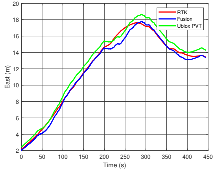
(a) East component of the rover position
