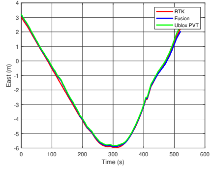
(a) East component of the rover position
