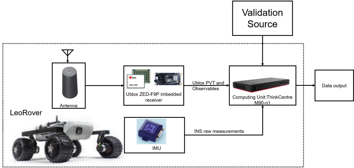
Figure 5: Architecture of the testing rig
