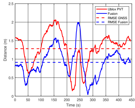
(c) Absolute distance
