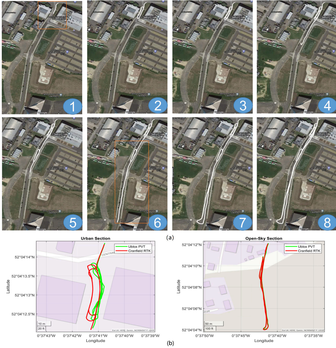
Figure 6: Illustration of the designed trajectory
