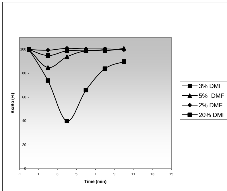
Figure 1: The effect of increasing concentrations of N,N-Dimethylformamide (DMF) on the biosensor response. FIA conditions: flow rate: 0.5 \text{ mL min}^{-1} ; injection loop: 1 mL. B_x/B_o (%), where B_x is the sample/standard maximum sensor output signal, and B_o is the original baseline.
