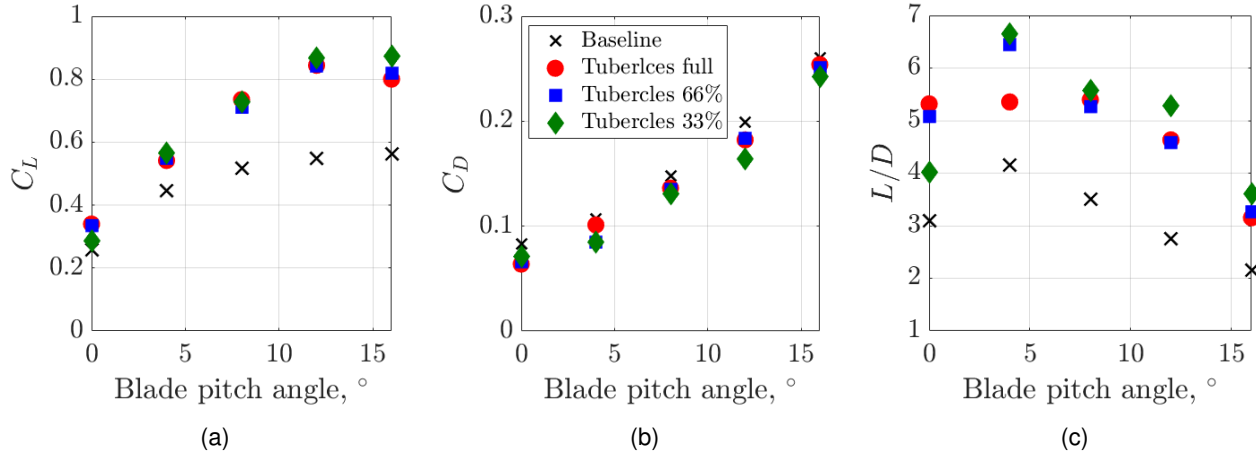
Figure 7 – Comparison of Lift and Drag Characteristics for the blade at zero sweep with and without full tubercles. U=36\text{m/s} ( \text{Rec} = 1.44 \times 10^5 ), sweep angle 0^\circ .
