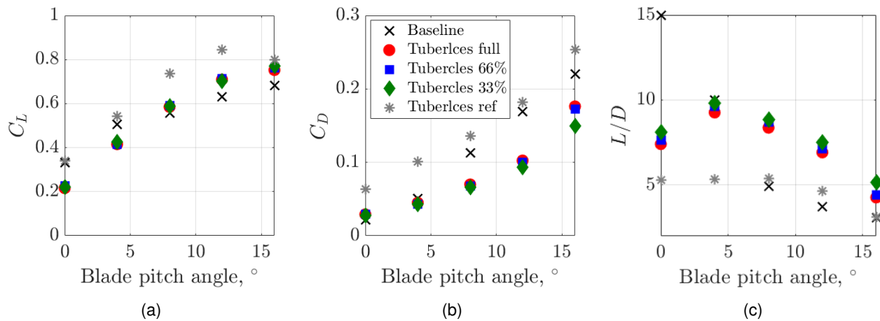
Figure 8 – Comparison of Lift and Drag Characteristics for the blade at zero sweep with and without full tubercles. U=36\text{m/s} ( \text{Rec} = 1.44 \times 10^5 ), sweep angle 30^\circ .
