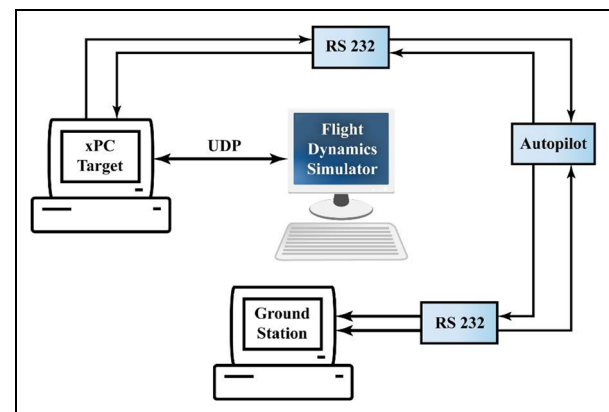
Figure 23. The HIL simulation system Structure adapted from. 137
