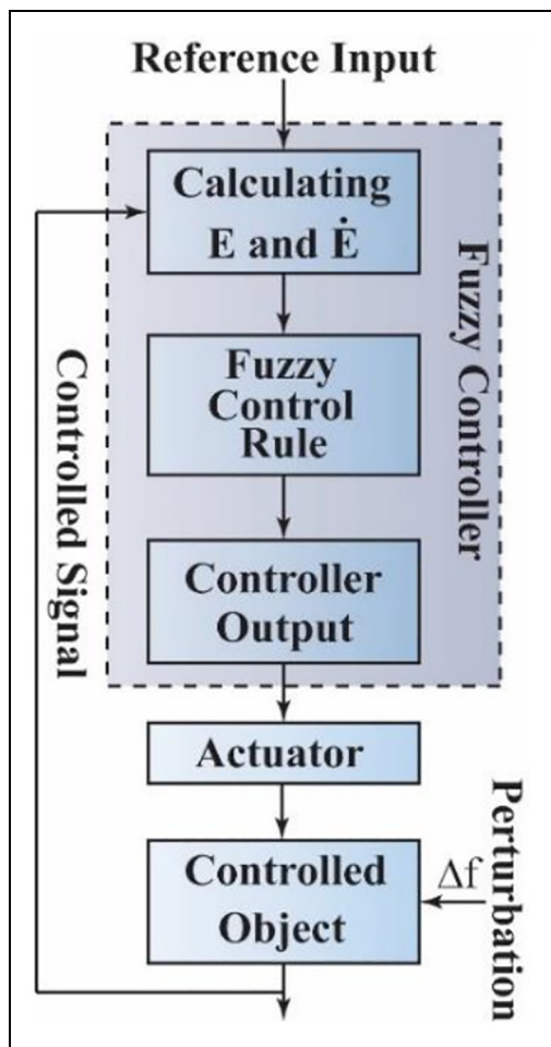
Figure 11. Principals of the fuzzy controller adapted from. 127
