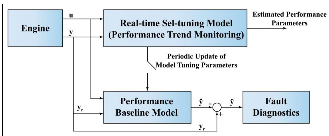
Figure 17. An integrated architecture for monitoring and fault diagnostics of aircraft engine performance adapted from. 112
