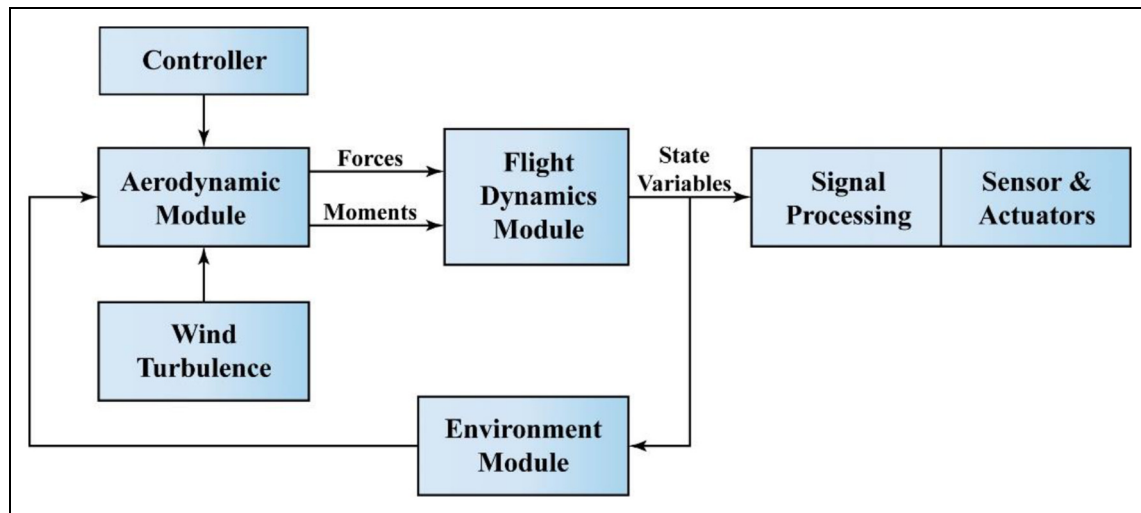
Figure 22. The UAV simulation model Structure adapted from. 137
