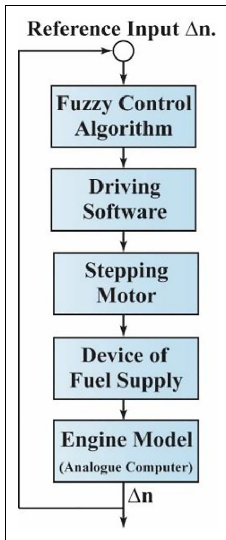
Figure 12. Block diagram of a simulation test adapted from. 127
