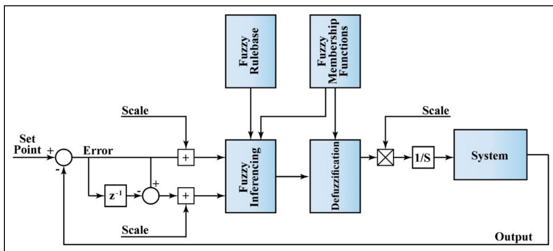
Figure 16. Closed-loop control system configuration adapted from. 132
