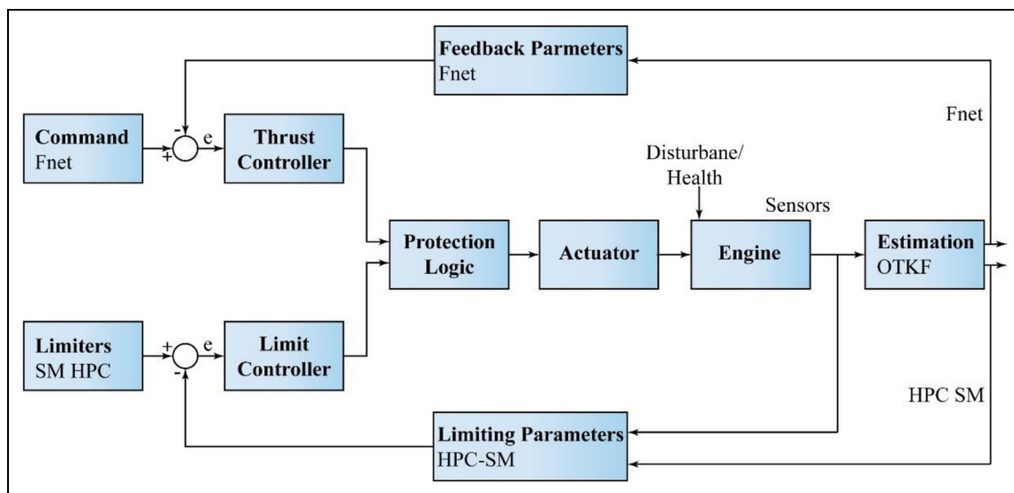
Figure 18. An architecture for model-based engine control to provide thrust and stall margin tight control adapted from. 112
