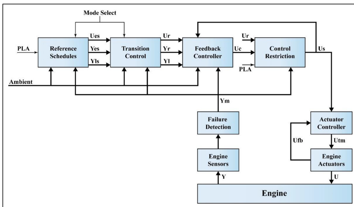
Figure 15. Structure of the main controller adapted from. 130
