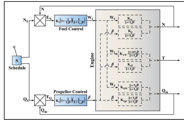
Figure 9. Engine control combination schematic diagram adapted from. 113
