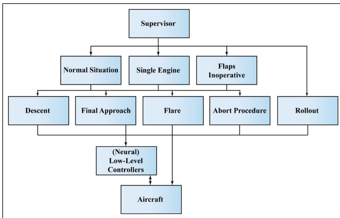
Figure 14. General layout of the controller structure adapted from. 129
