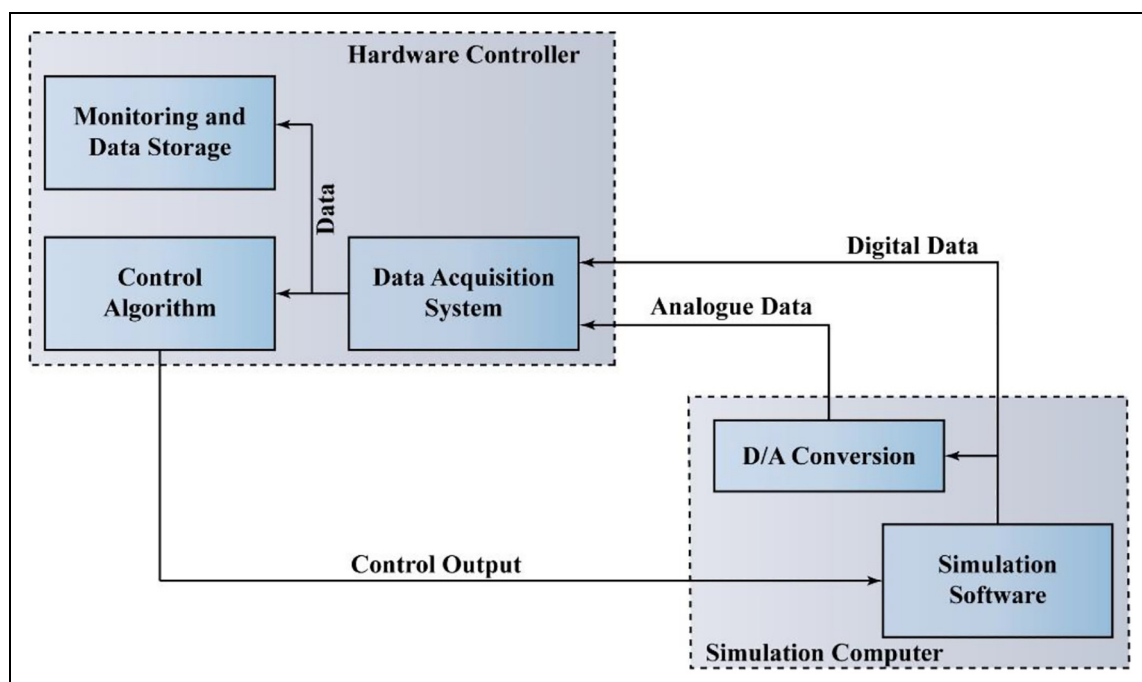
Figure 13. Test facility of hardware in the loop adapted from. 128
