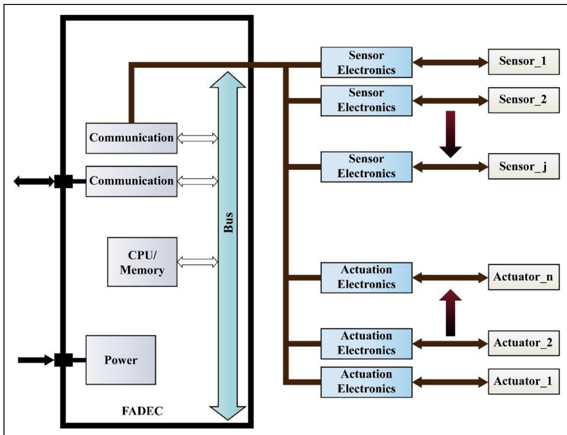
Figure 20. Distributed engine control adapted from. 112
