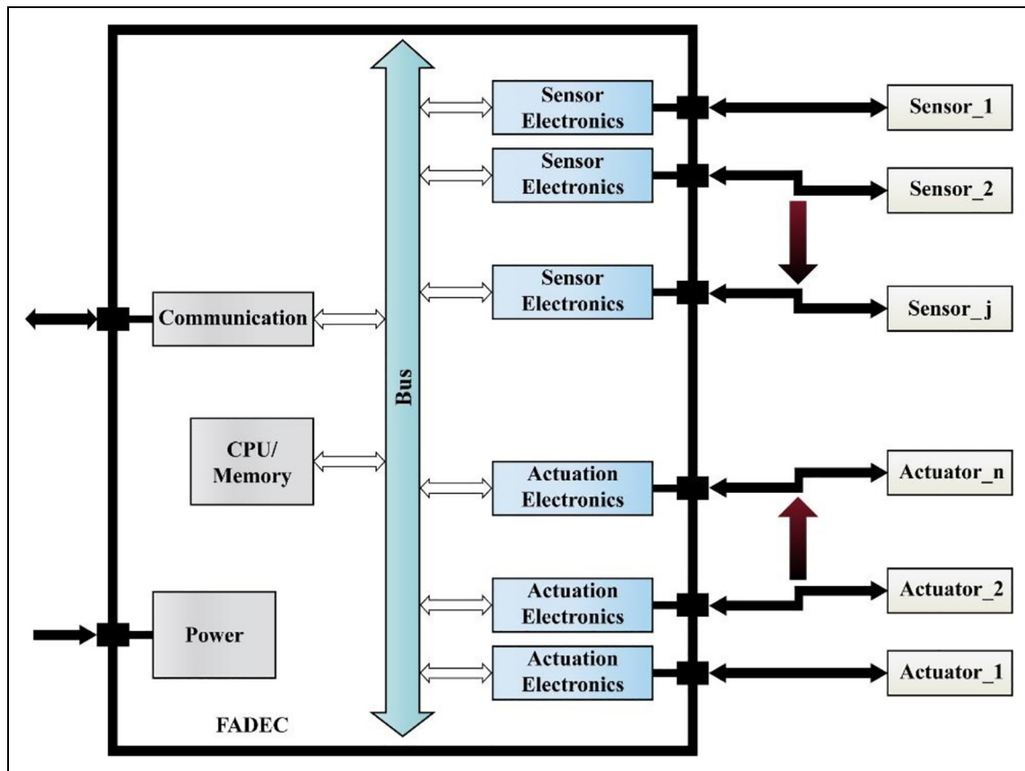
Figure 19. Centralized engine control adapted from. 112
