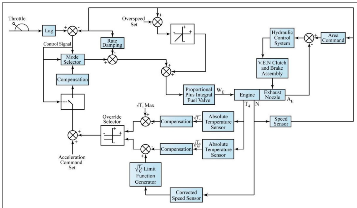
Figure 10. Block diagram of fluidic controller adapted from. 116
