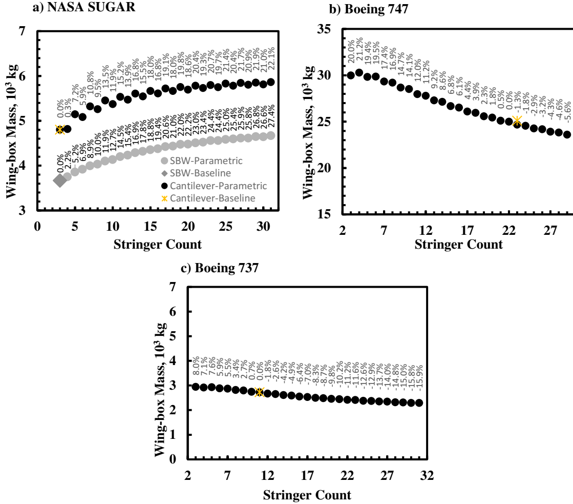
Fig. 8 a) a) NASA SUGAR-SBW, SUGAR-CANT; b) Boeing 747; c) Boeing 737: baseline aircraft wing-box mass variation with total stringer counts.
