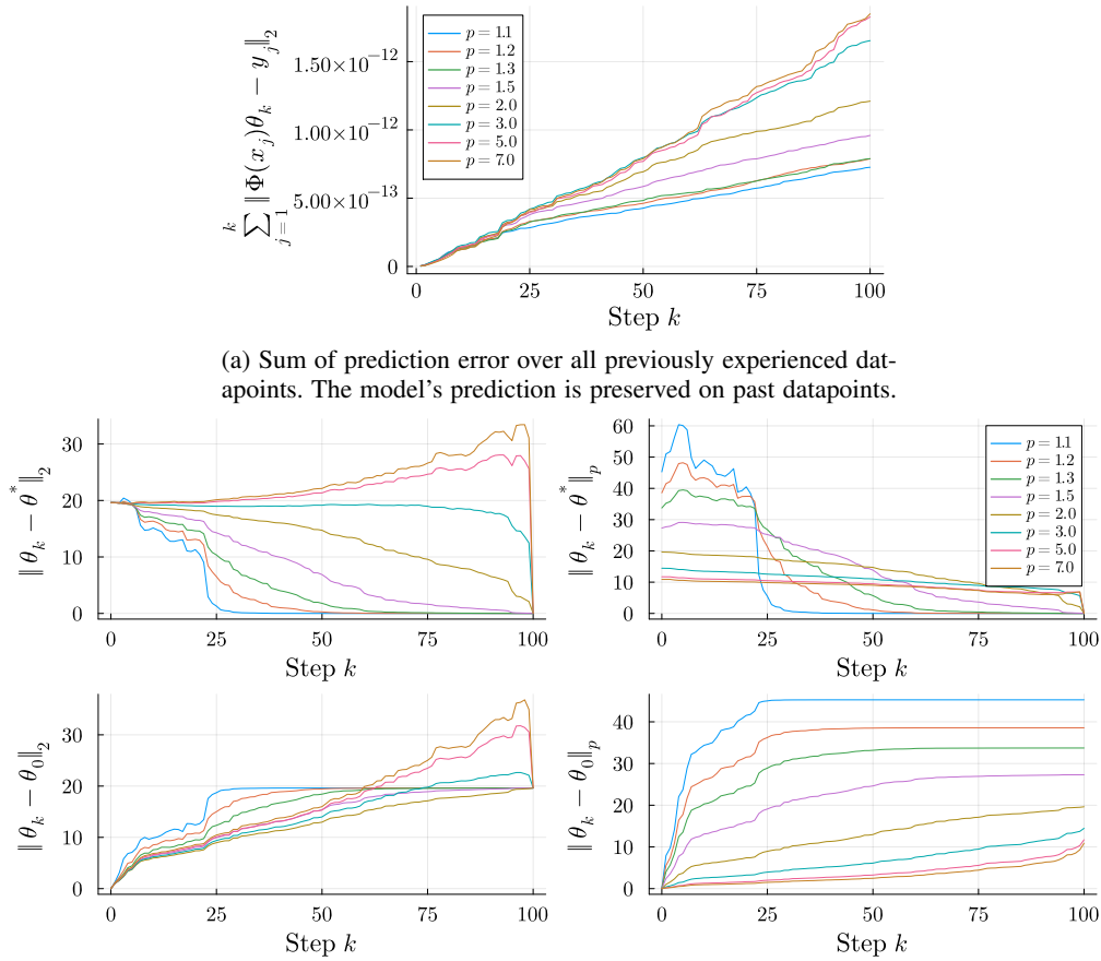
(b) Parameter estimation error (1st row) and deviation from initial value (2nd row). Smaller p results in earlier and smoother convergence. Large p leads to abrupt correction as soon as the parameter can be uniquely determined.
