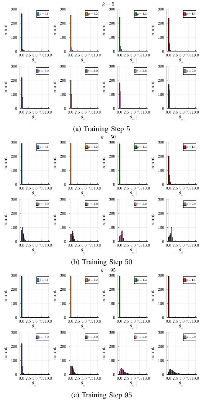
Fig. 3: Snapshots of the histogram for the elementwise absolute value of parameters at training steps k = 5, 50, 95 . p close to 1 promotes sparsity of the learned parameters.
