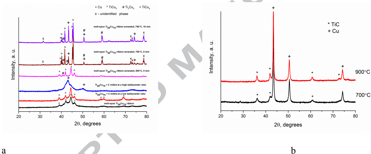
Fig. 1. XRD patterns of (a) melt-spun Ti_{25}Cu_{75} alloy ribbons, powders obtained by ball milling of the ribbons with carbon, and annealed ribbons (the holding time at the maximum temperature is given); (b) sintered TiC-Cu nanocomposites.
