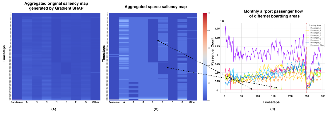
Figure 3.3: Readability comparison of saliency visualisations (heatmaps of the same tensors): (A) aggregated original saliency tensor A ; (B) aggregated sparse saliency tensor A' ; (C) monthly passenger flow for San Francisco Airport boarding areas.
