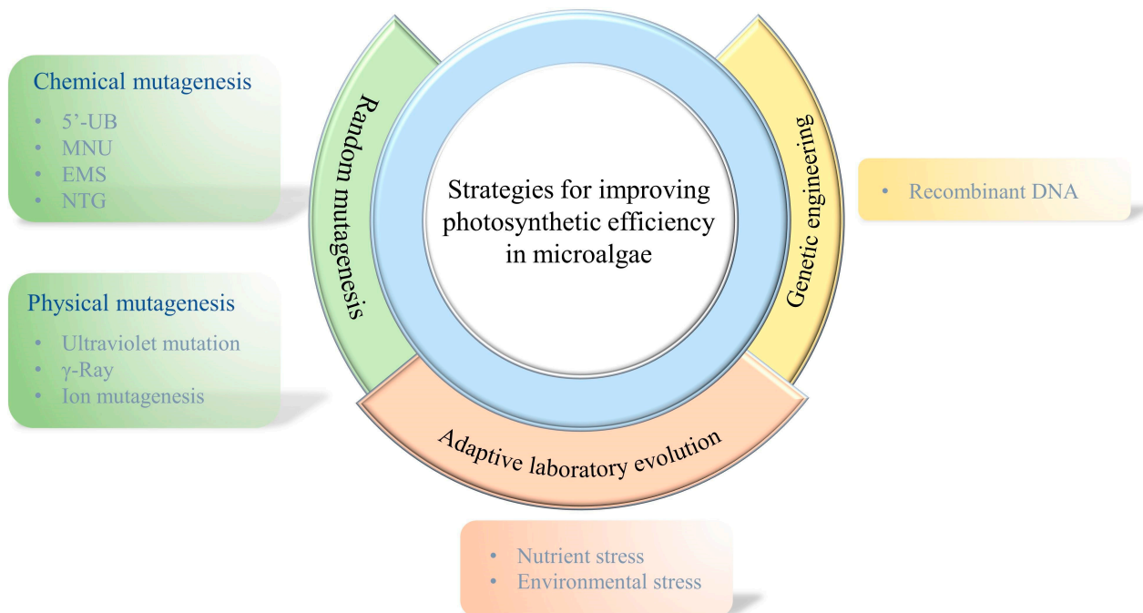
Figure 6. Strategies for improving photosynthetic efficiency in microalgae.
