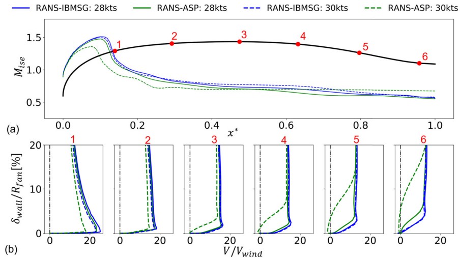
Fig. 12. (a) Isentropic Mach number profiles and (b) streamwise velocity profiles for the aspirated and powered (IBMSG) configurations at \phi = 90^\circ .
