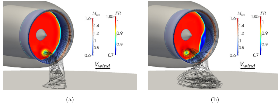
Fig. 6. (a) Critical ( V_{wind} = 28kts ) and (b) post-critical ( V_{wind} = 30kts ) conditions for the aspirated intake configuration (RANS-ASP).
