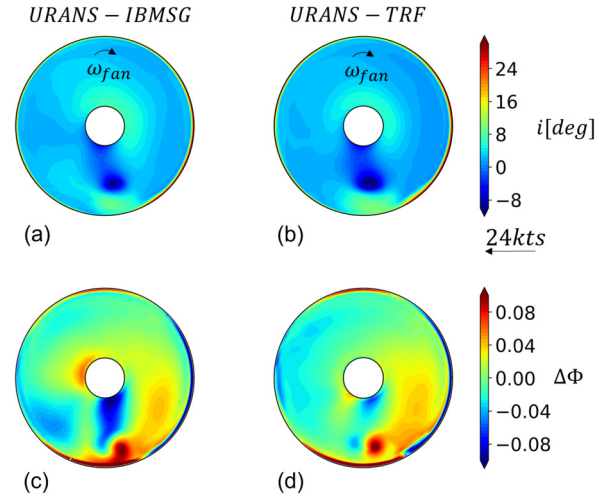
Fig. 23. (a), (b) Time average blade incidence angle ( i ) and (c), (d) time average flow coefficient deviation ( \Delta\Phi ) distributions at the AIP at V_{wind} = 24\text{ kts} .
