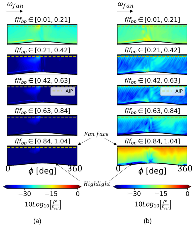
Fig. 22. Banded Fourier spectra of static pressure fluctuations on the intake surface. (a) URANS-IBMSG and (b) URANS-TRF at V_{wind} = 24\text{ kts} .
