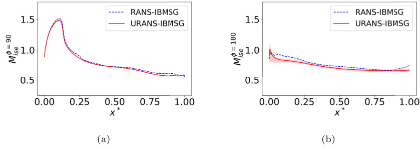
Fig. 13. Isentropic Mach number profiles at (a) \phi = 90^\circ and (b) 180^\circ for the steady and unsteady powered (IBMSG) configuration at V_{wind} = 28kts . The shaded region refers to URANS-IBMSG and marks the max and minimum values through-out the fan revolutions.
