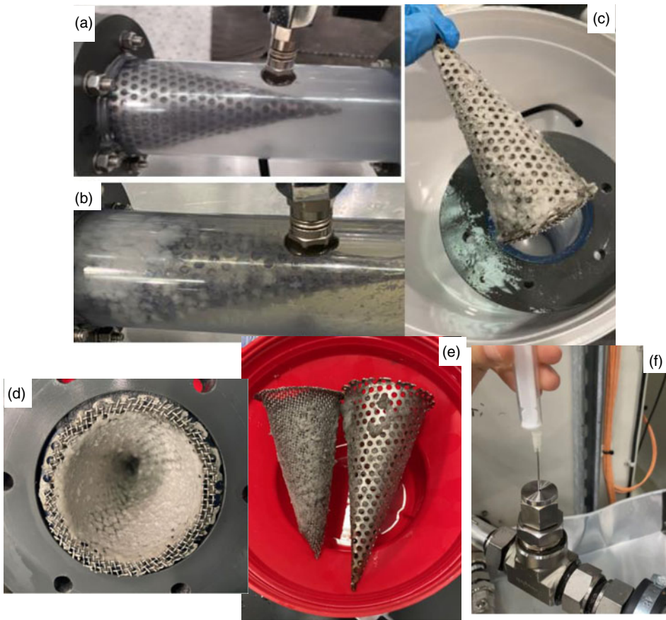
Figure 3. Strainer section in flowing fuel at; (a) room temperature and; (b) after an icing experiment; (c) strainer section removed after an icing experiment; (d) after an icing experiment (inside view); (e) after an icing experiment, removable mesh and outer support cone; (f) fuel sample point.
