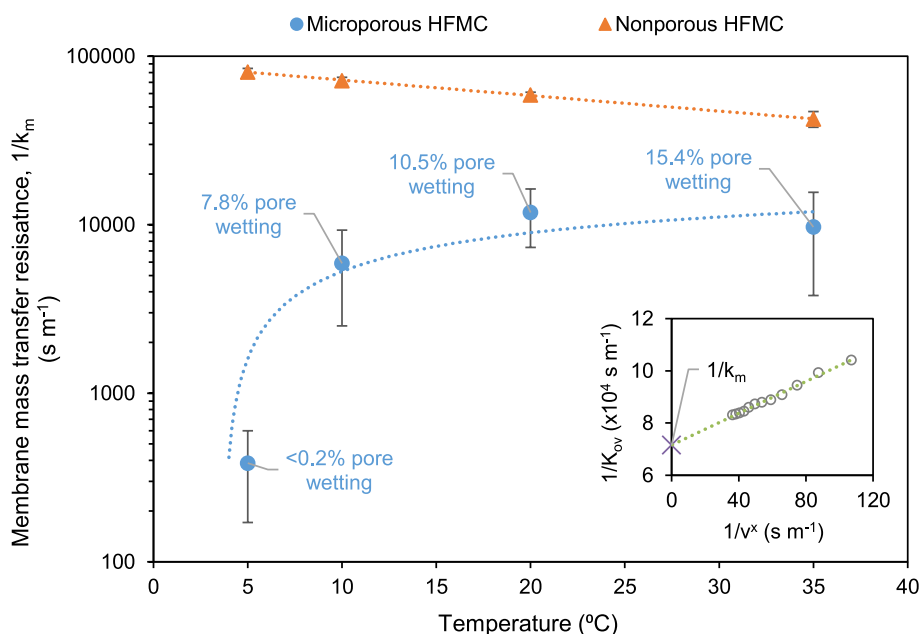
Fig. 3. Impact of solvent temperature on membrane mass transfer resistance for \text{CO}_2 within microporous (PP) and nonporous (PMP) membranes. Membrane mass transfer resistances determined using Wilson plot method (example inset for nonporous membrane at 10^\circ\text{C} ). Conditions: Pure \text{CO}_2 gas feed; v_G = 0.07\text{--}0.08 \text{ m s}^{-1} ; P_g = 1.1 \text{ bar} ; gas temperature in = 21^\circ\text{C} . Estimated pore wetting annotated (Equation (6)). Dotted lines added to guide the eye.
