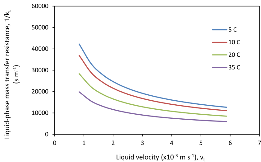
Fig. B1. Projected impact of temperature on liquid-phase mass transfer resistance for \text{CO}_2 transport from the liquid-membrane interface to the liquid bulk for the (a) microporous, and (b) nonporous membranes (Equation (5)).
