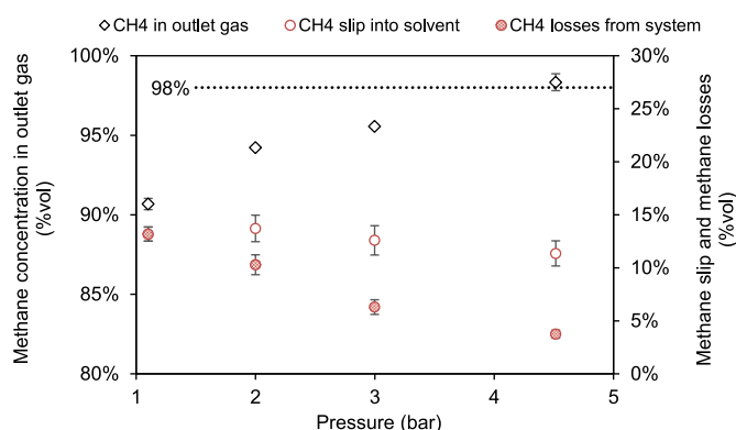
Fig. 11. Impact of gas pressure on outlet gas quality, methane slip and methane losses from the system in the microporous module. Conditions: 50:50 CO 2 /CH 4 gas feed, v_G = 0.02 m s -1 , v_L = 1.7 \times 10^{-3} m s -1 ; solvent temperature = 5–10 °C; gas temperature in = 21 °C. Ideal dissolved methane recovery estimated for solvent depressurisation to 1.5 bar in a flash vessel. Absolute pressure values provided.
