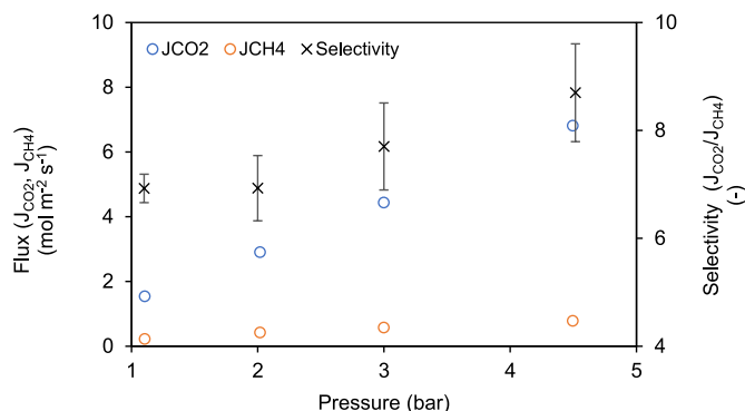
Fig. 10. Influence of pressure on the selectivity of CO 2 transport within the microporous membrane. Conditions: 50:50 CO 2 /CH 4 gas feed; v_G = 0.02 m s -1 , L/G = 1.4; v_L = 1.7 \times 10^{-3} m s -1 ; solvent temperature = 5–10 °C, gas temperature in = 21 °C. Absolute pressure values provided.
