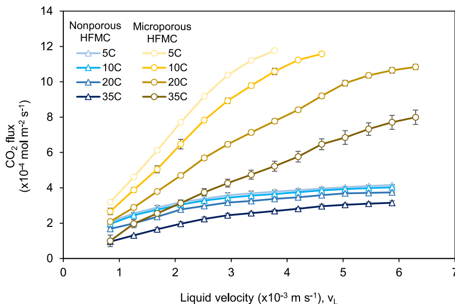
Fig. 2. Impact of solvent temperature on \text{CO}_2 flux across microporous (PP) and nonporous (PMP) membranes. Conditions: Pure \text{CO}_2 gas feed; v_G = 0.07\text{--}0.08 \text{ m s}^{-1} ; P_g = 1.1 \text{ bar} ; gas temperature in = 21^\circ\text{C} .
