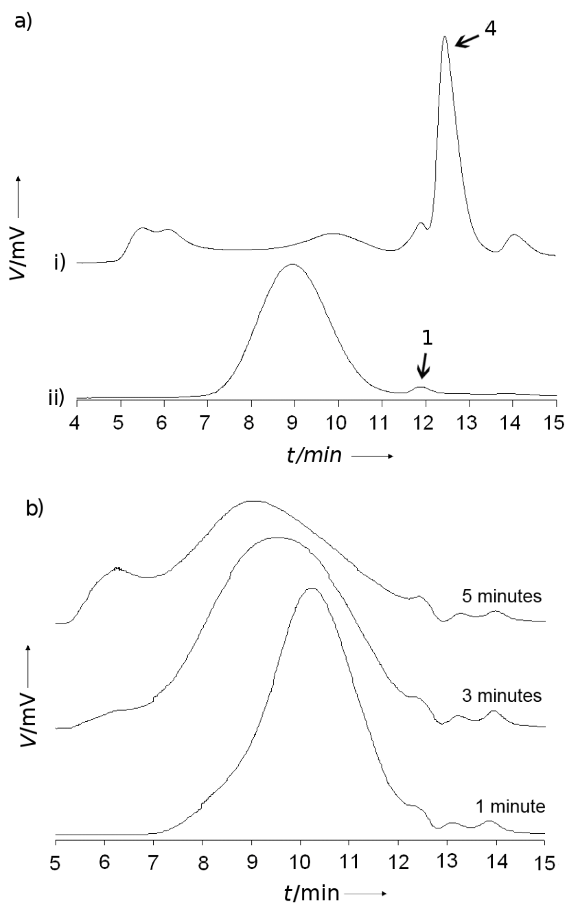
Figure 2. GPC curves for: a) 2 (i) and 3 supernatant (ii); b) samples taken from the initial stages of the photochemical crosslinking reaction.
