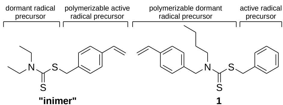
Scheme 1. The structure of Otsu's "inimer"[8] (left) and of the monomer used in this work: benzyl N -butyl- N -(4-vinylbenzyl) dithiocarbamate, ( 1 ), or "reversed inimer" (right), showing the differences between the two structures with respect to the active and dormant radical precursor sites and the position of the polymerizable functionality.
